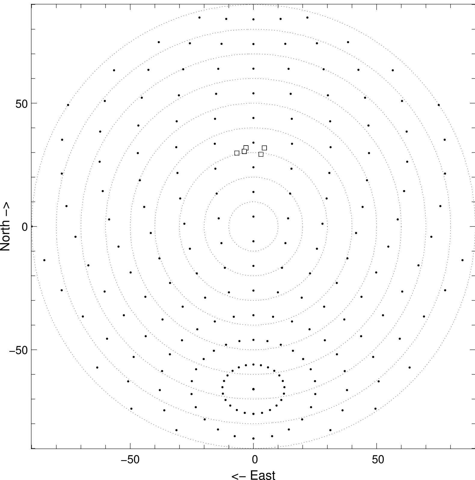
Trace of observations on Sky (obs at -24^{\circ} )
