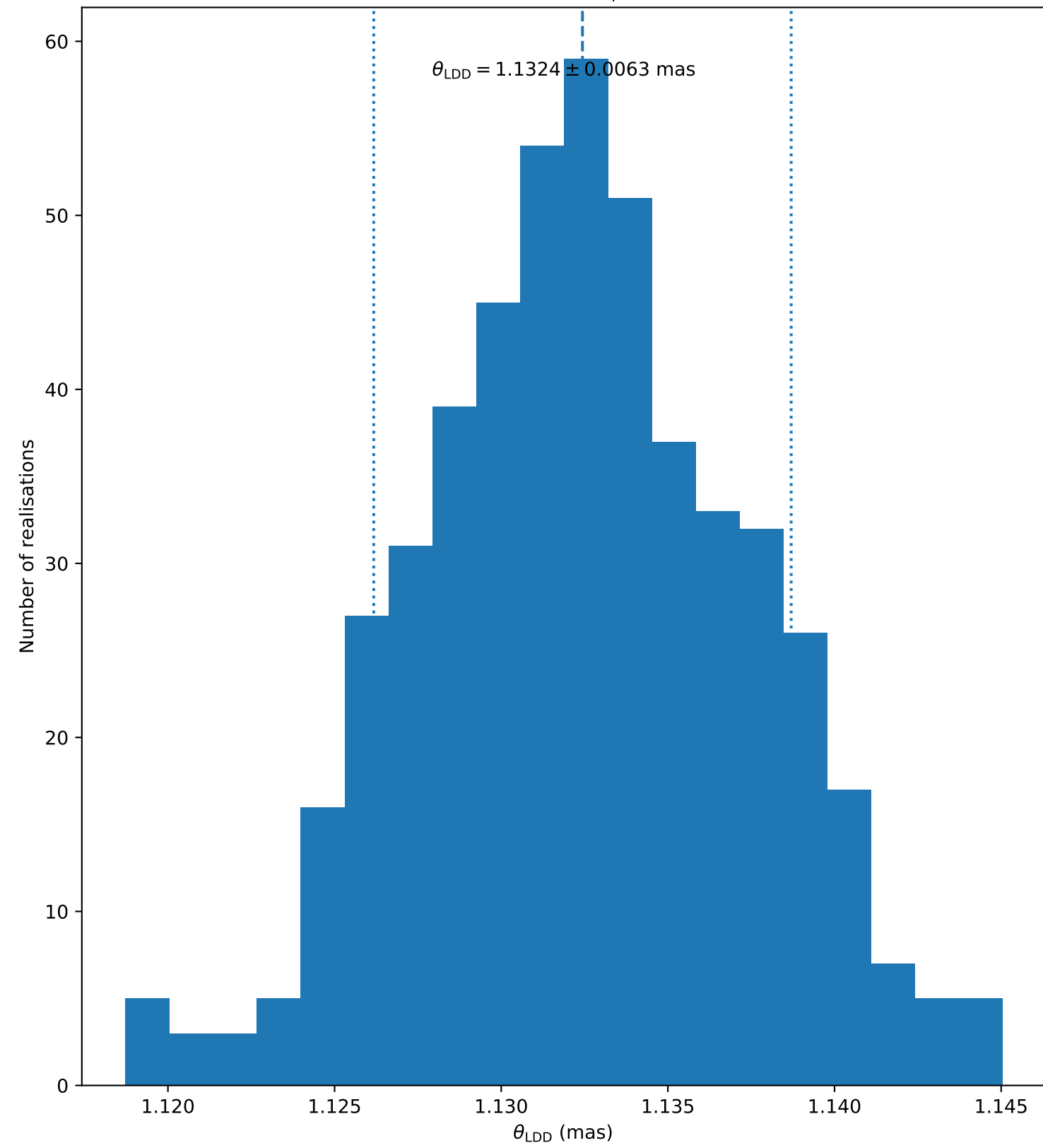
zet_Tuc ( N_{\text{bootstrap}} = 500 )
