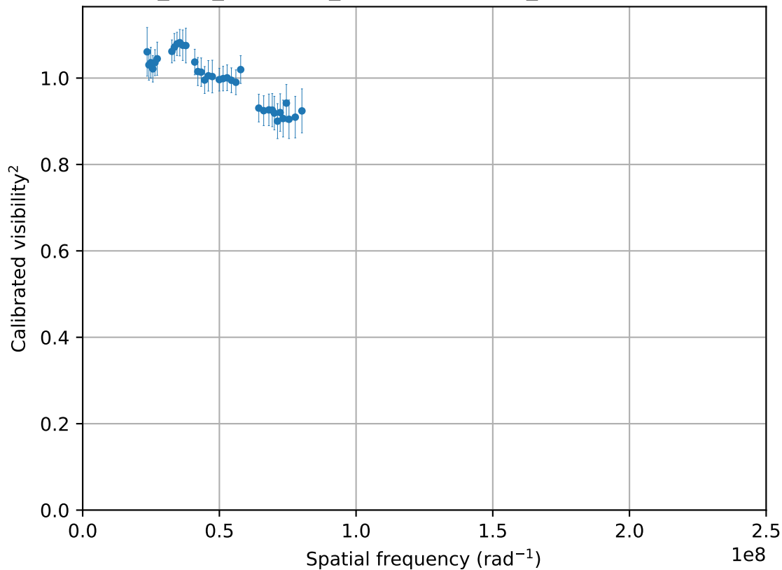
2019-11-25_CAL_HD65187_oidataCalibrated_499 (36 valid vis 2 points)
