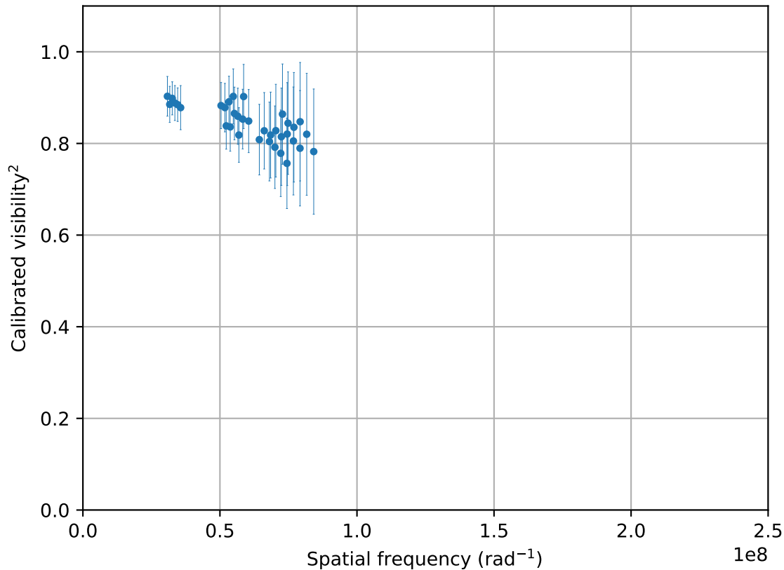
2019-11-28_CAL_HD30519_oidataCalibrated_499 (36 valid vis 2 points)
