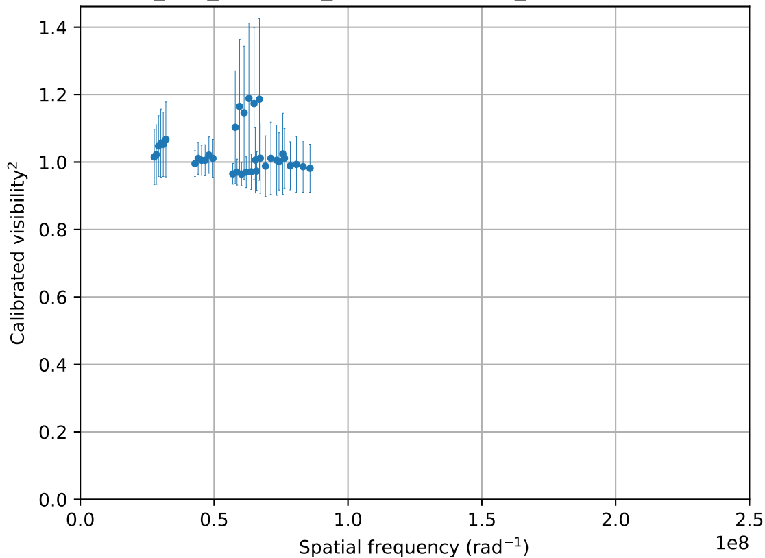
2021-02-18_CAL_HD38295_oidataCalibrated_499 (36 valid vis 2 points)
