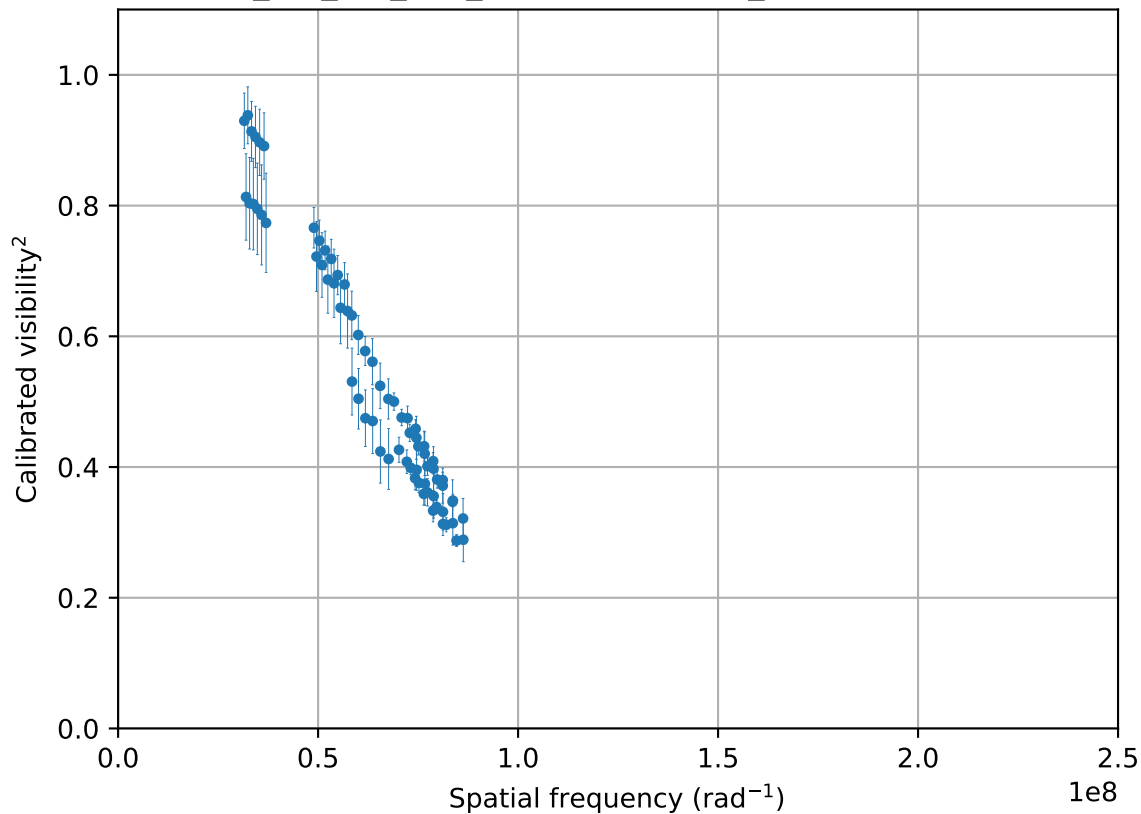
2021-02-18_SCI_rho_Pup_oidataCalibrated_499 (72 valid vis 2 points)
