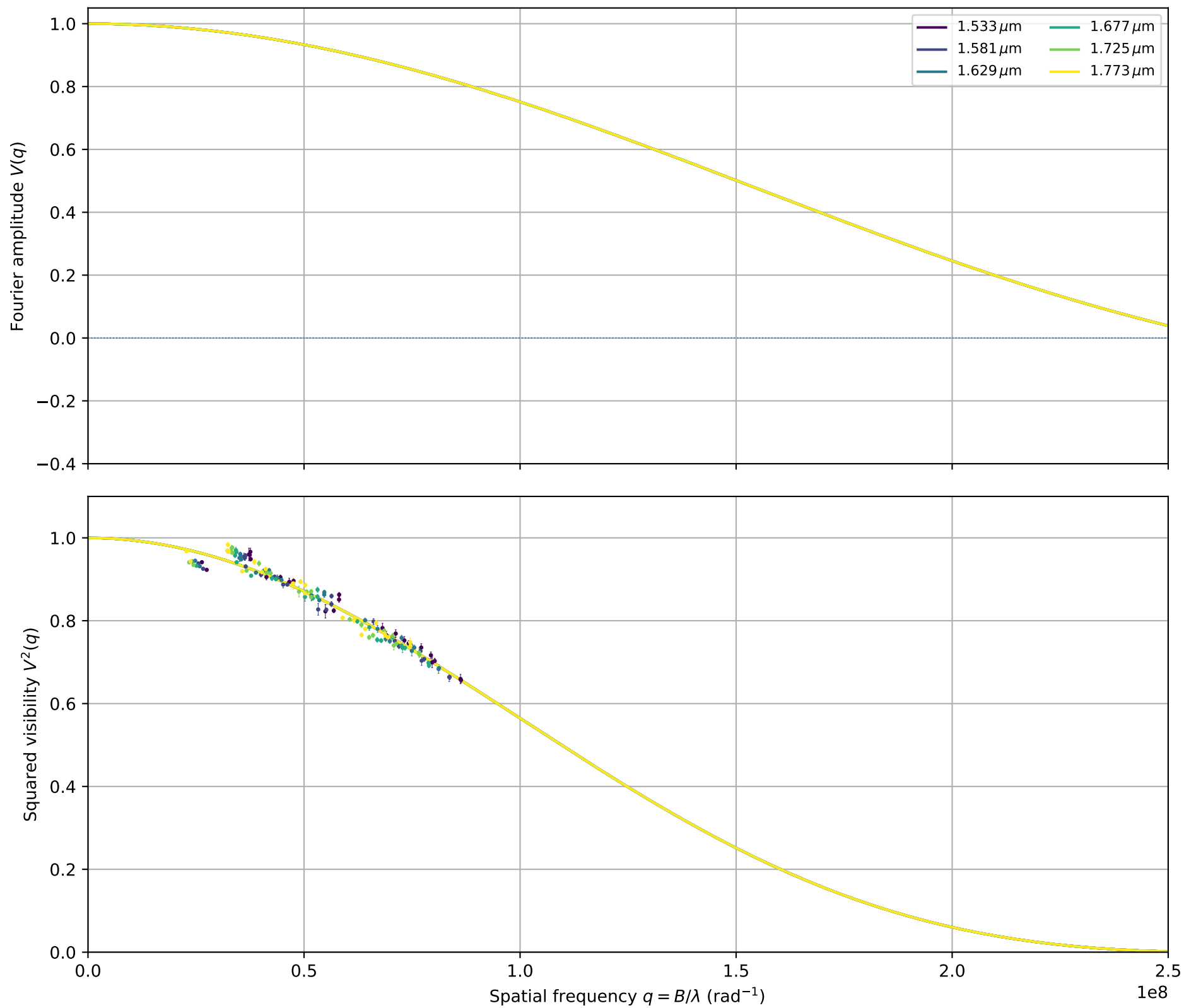
HR_2998: fitted \theta_{\text{LDD}} = 0.9918 \pm 0.0106 mas
