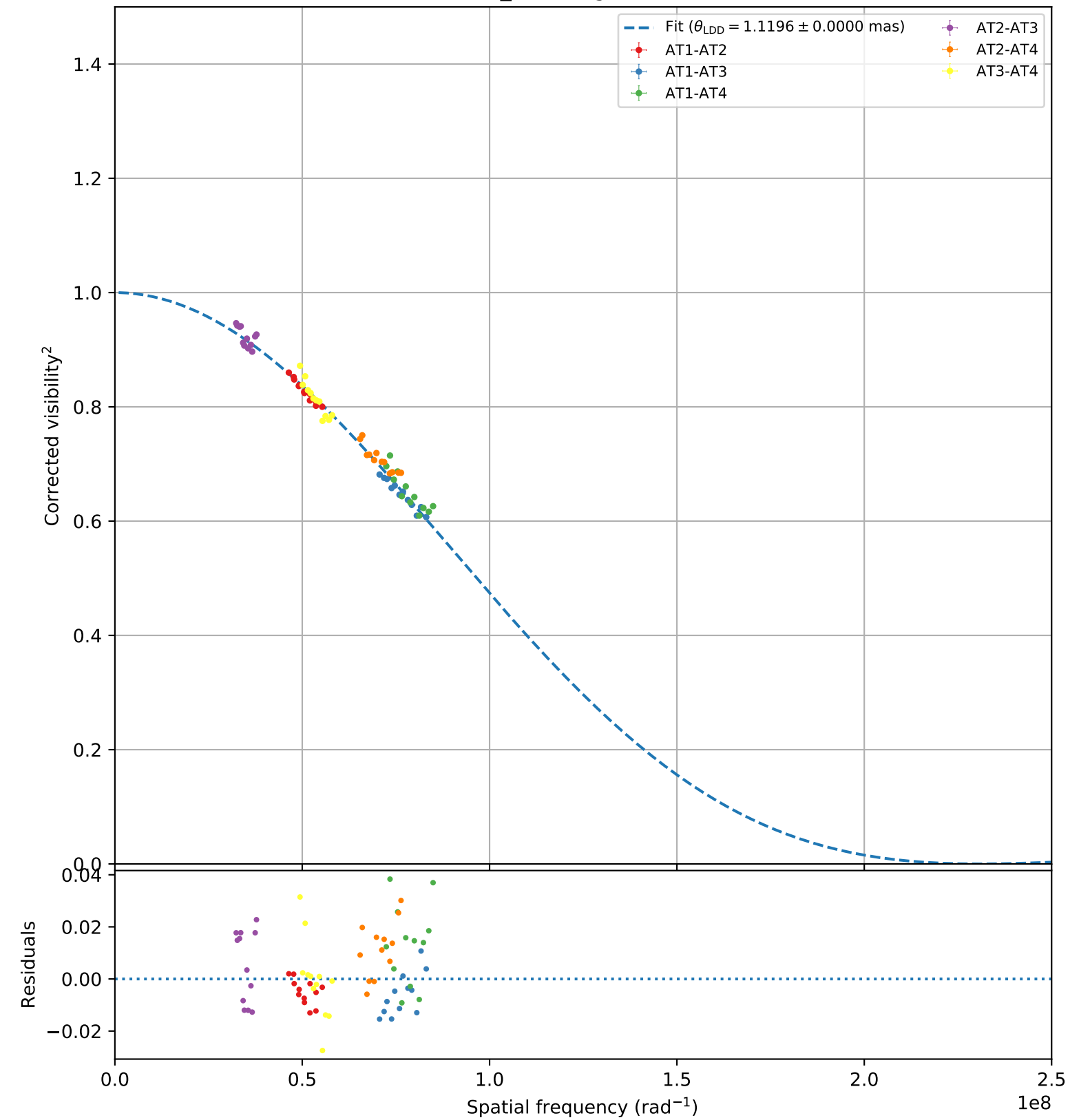
iot_Psc (bright, 104)
