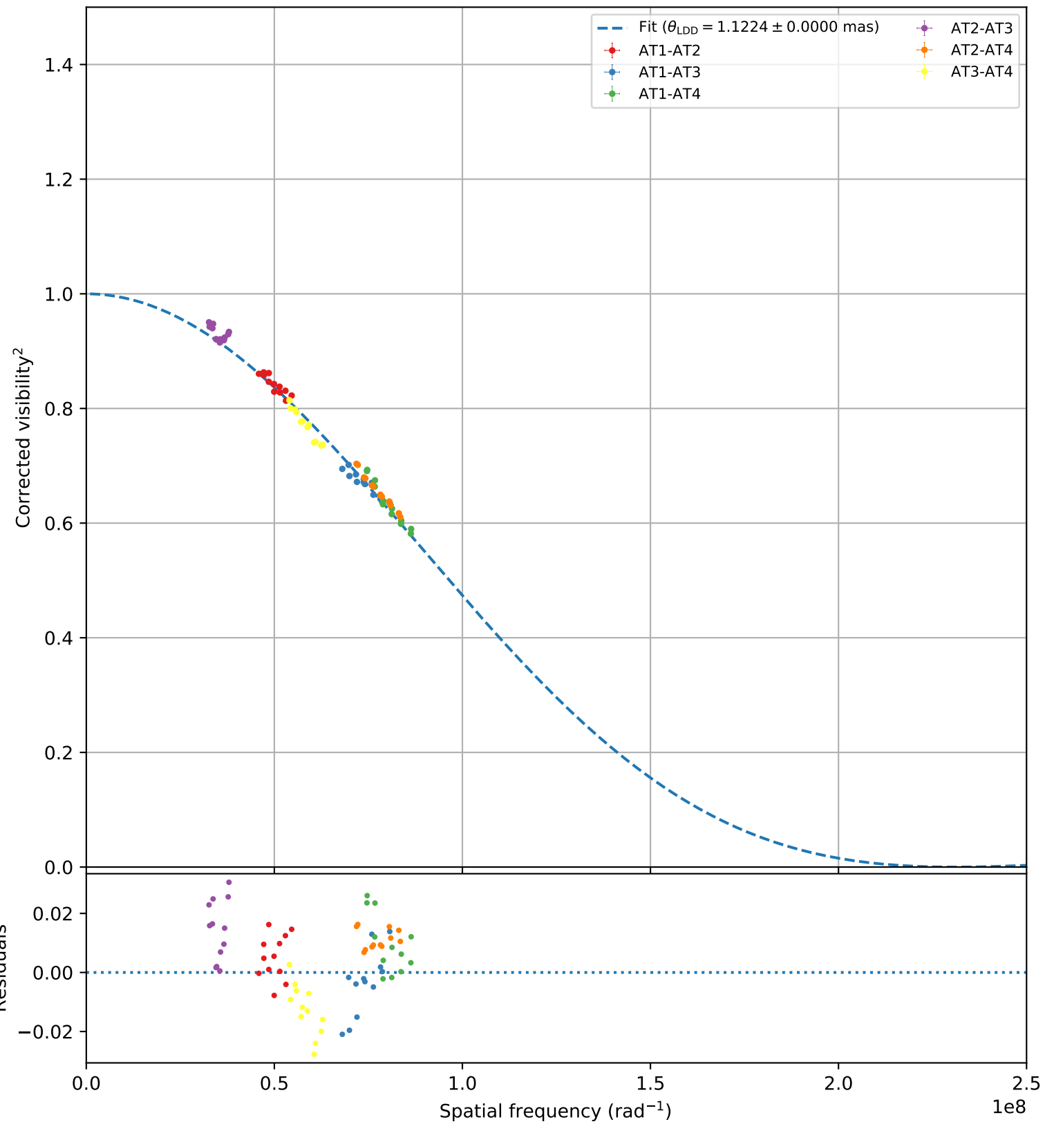
HD124850 (faint, 105)
