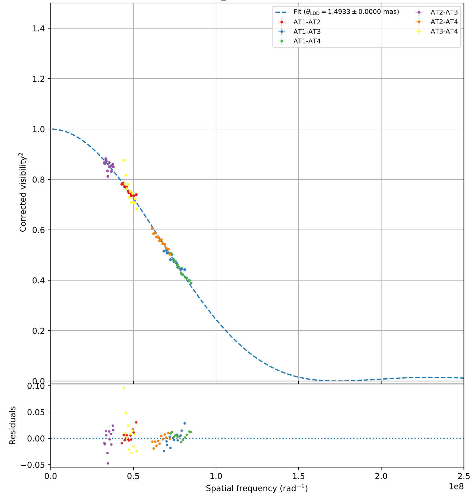
ksi_Gem (faint, 106)
