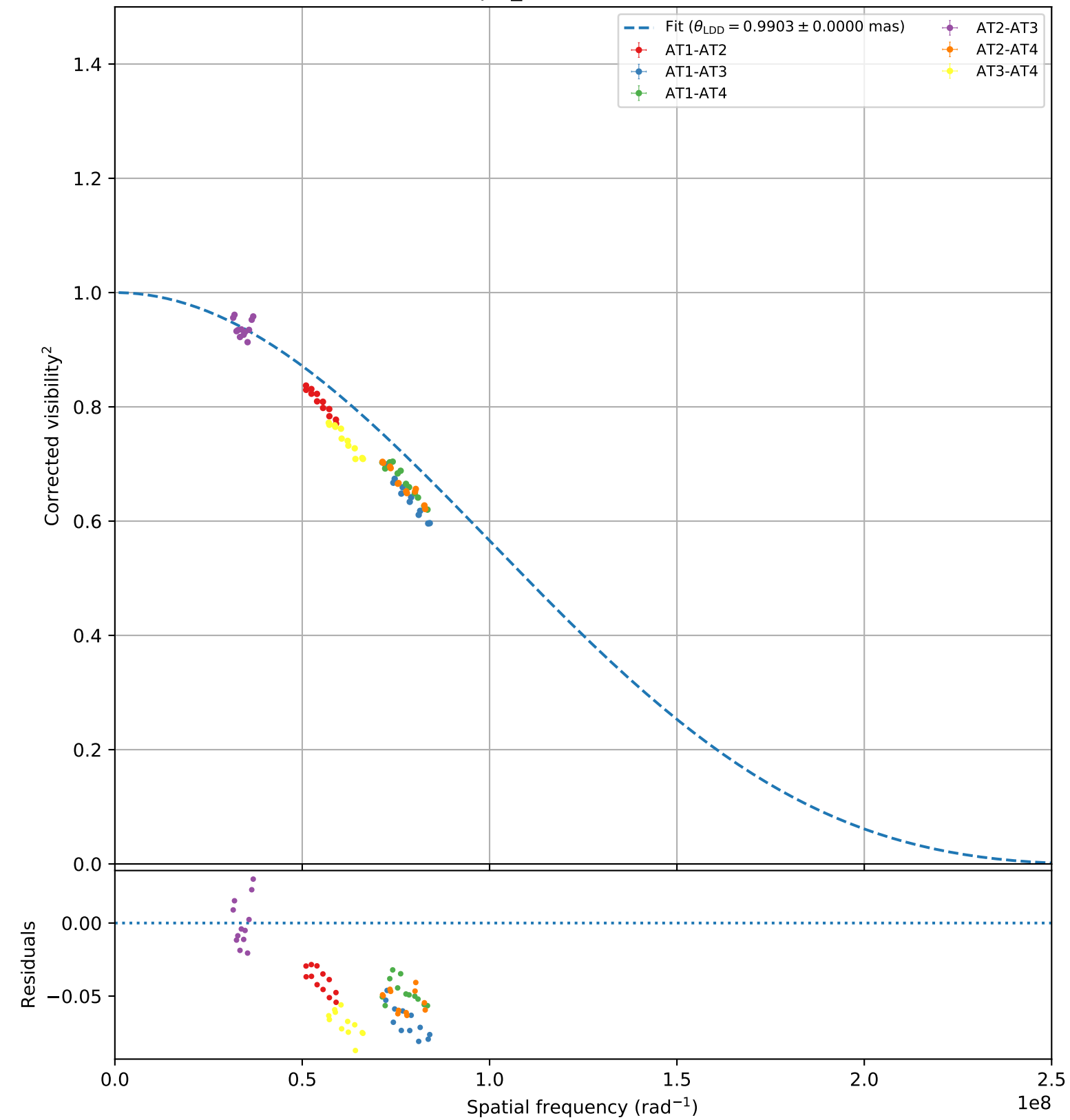
psi_Vel (faint, 106)
