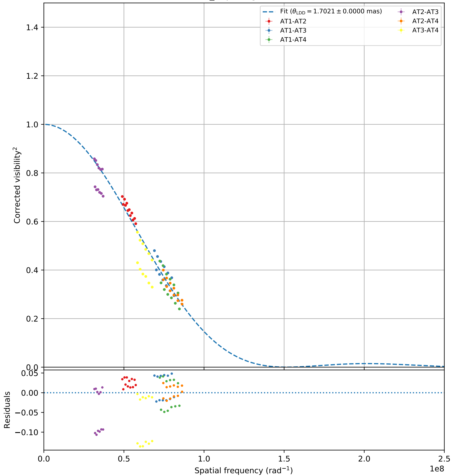
rho_Pup (bright, 106)
