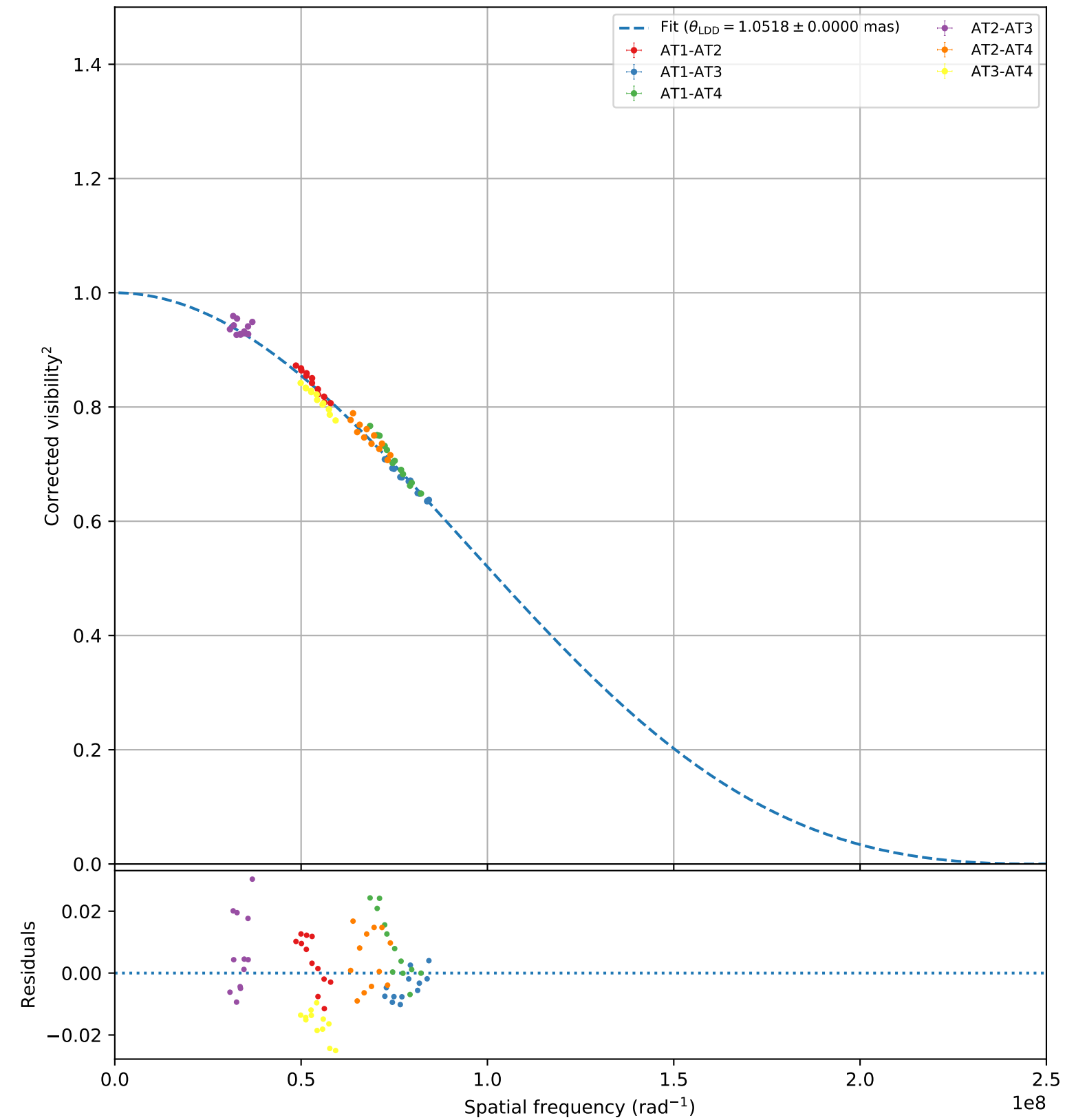
HD141004 (faint, 105)
