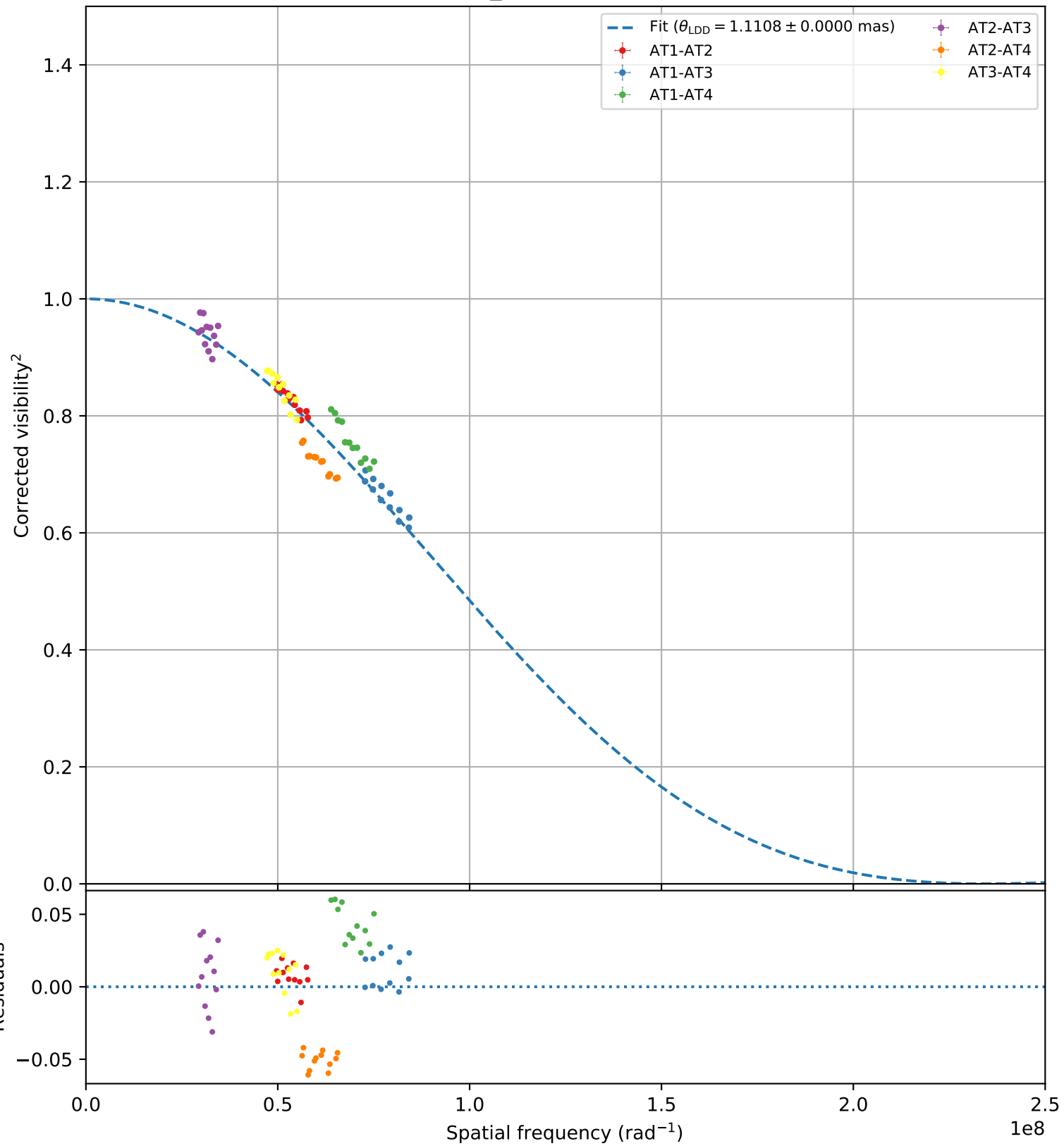
zet_Tuc (faint, 104)
