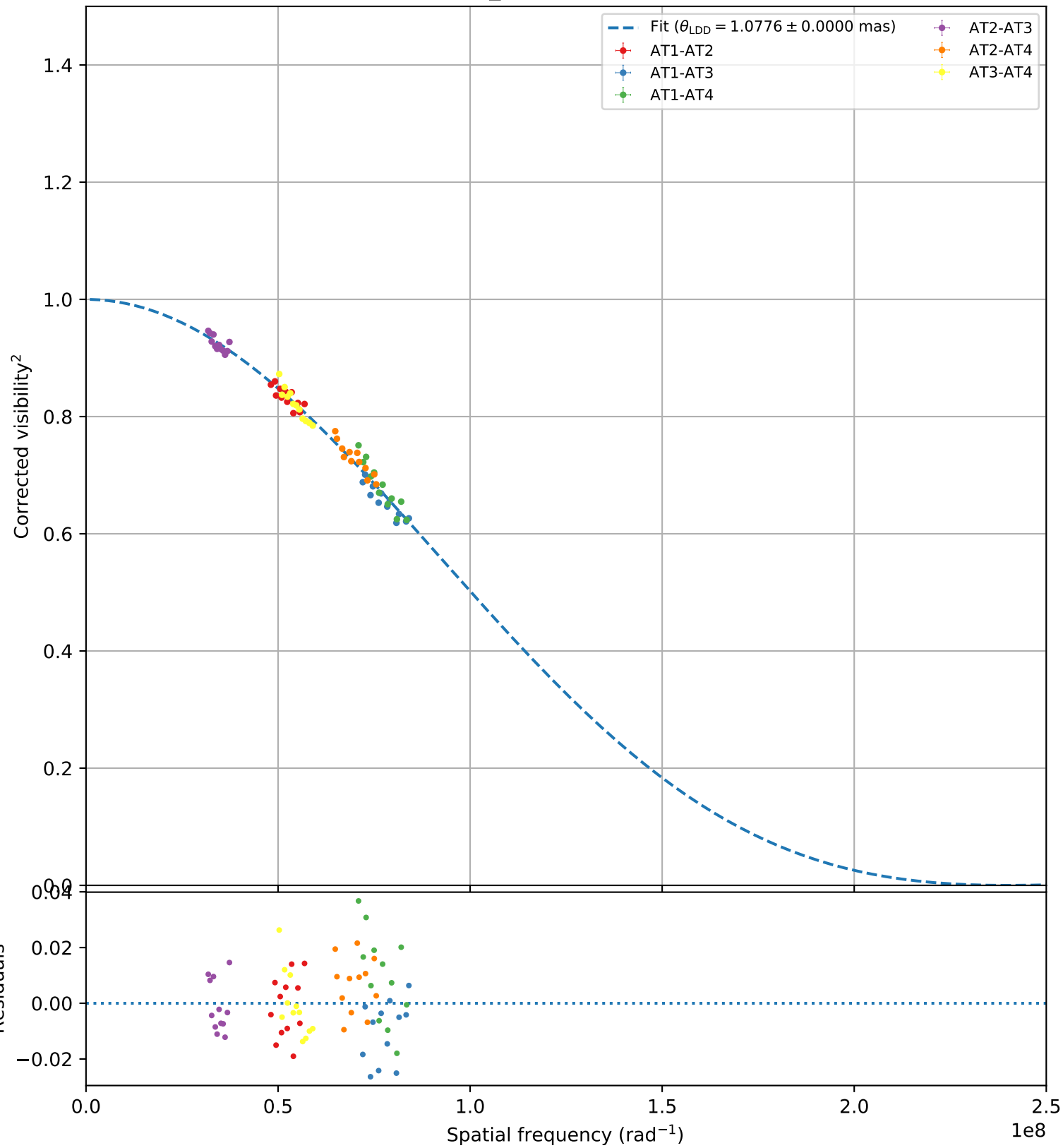
iot_Psc (faint, 104)
