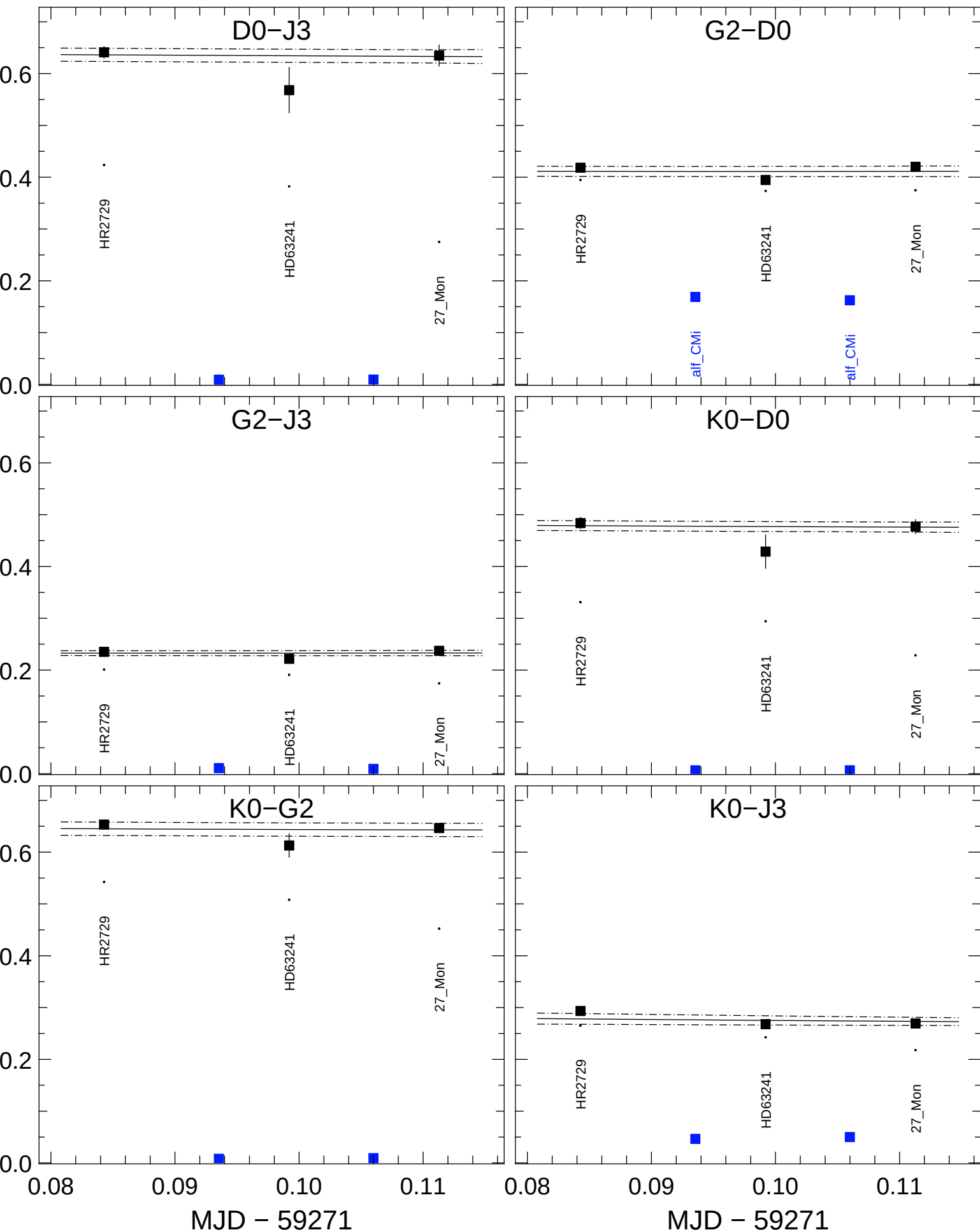
Transfer-Function vis2 (black) and Scientific vis2 (colors) averaged in the range [1.61782, 1.61782] \mu\text{m}
