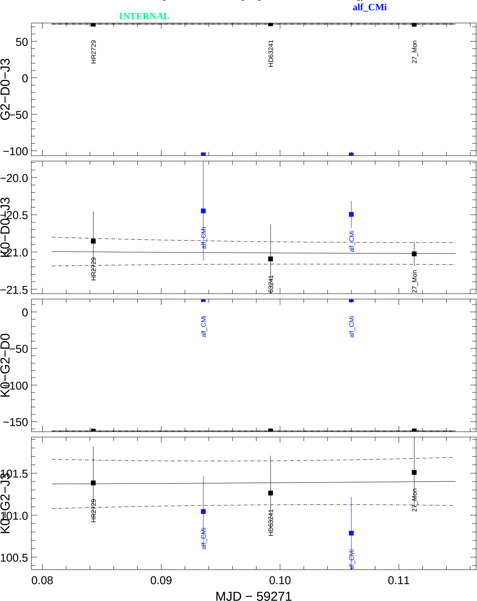
Transfer-Function t3Phi (black) and Scientific t3Phi (colors) averaged in the range [1.61782,1.61782] \mu\text{m}
