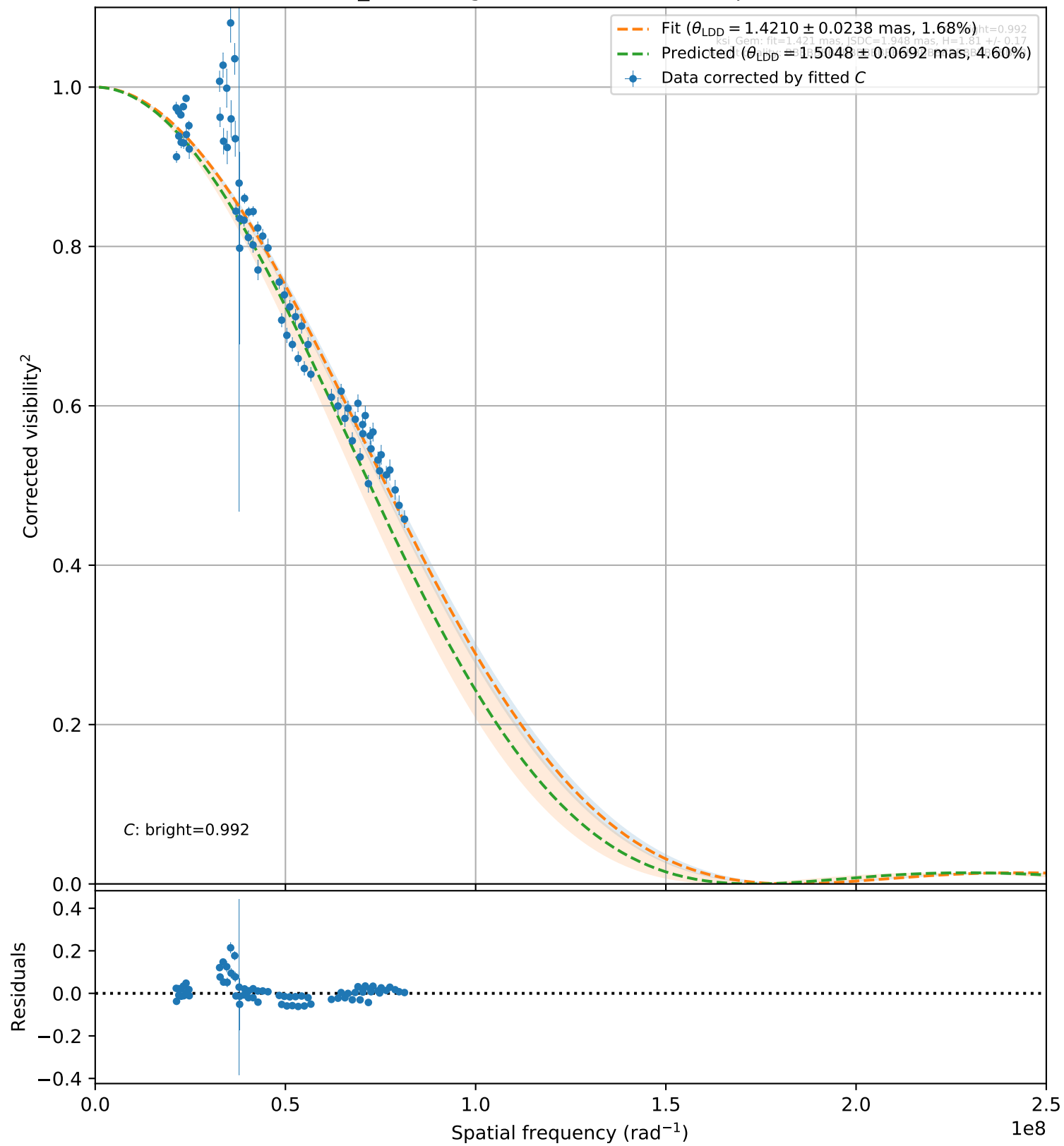
ksi_Gem (bright, 106) (72 valid vis 2 points)
