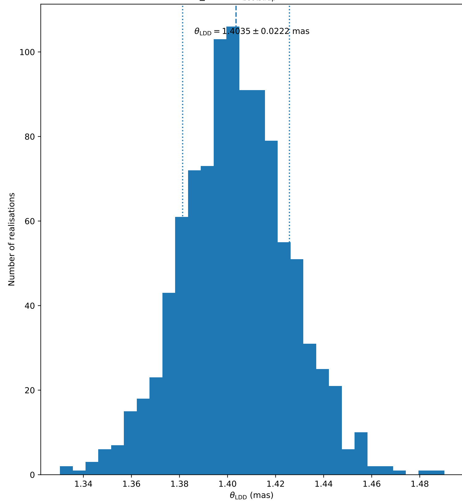
ksi_Gem ( N_{\text{bootstrap}} = 1000 )
