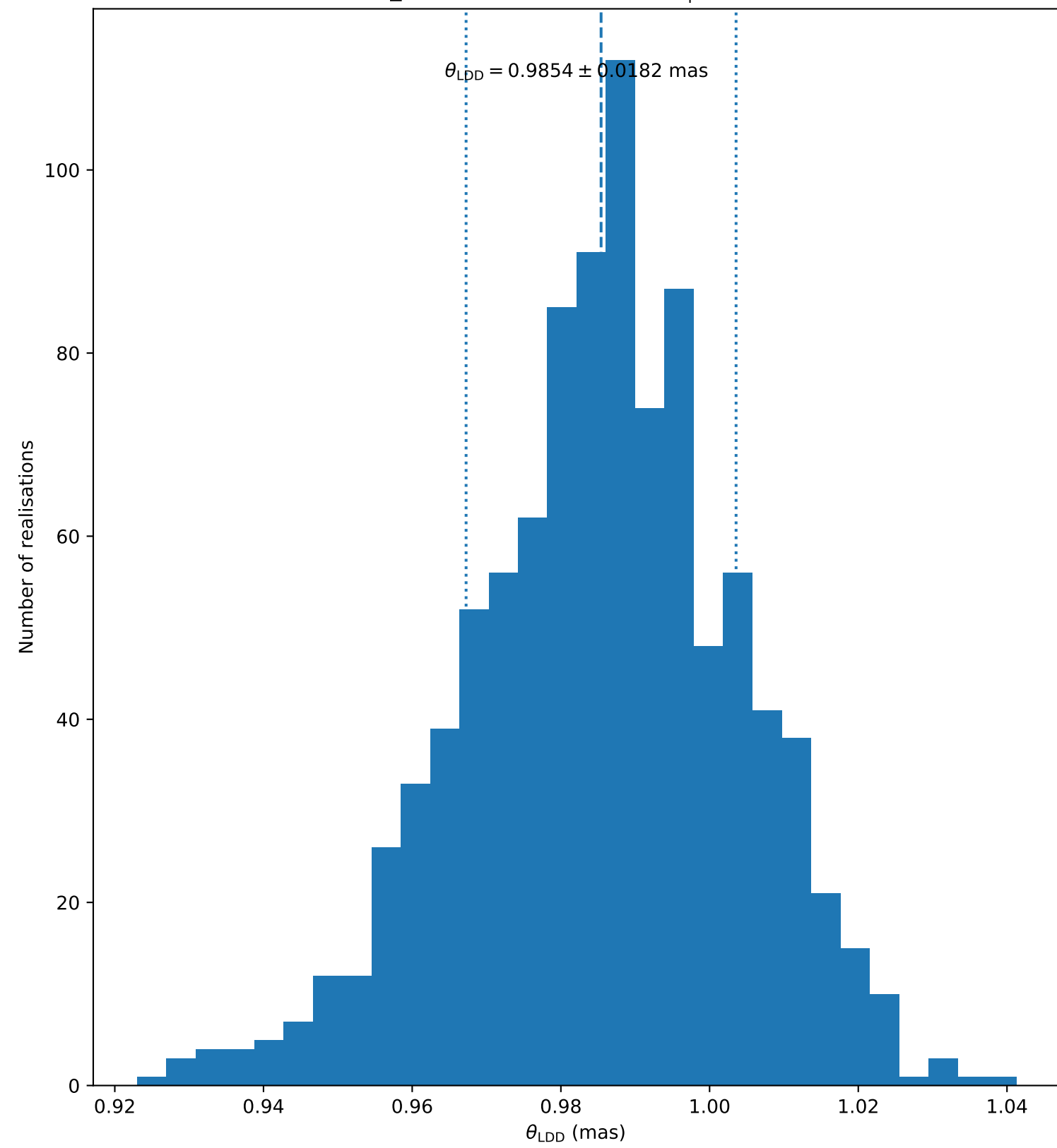
ksi_Gem (faint, 106) ( N_{\text{bootstrap}} = 1000 )
