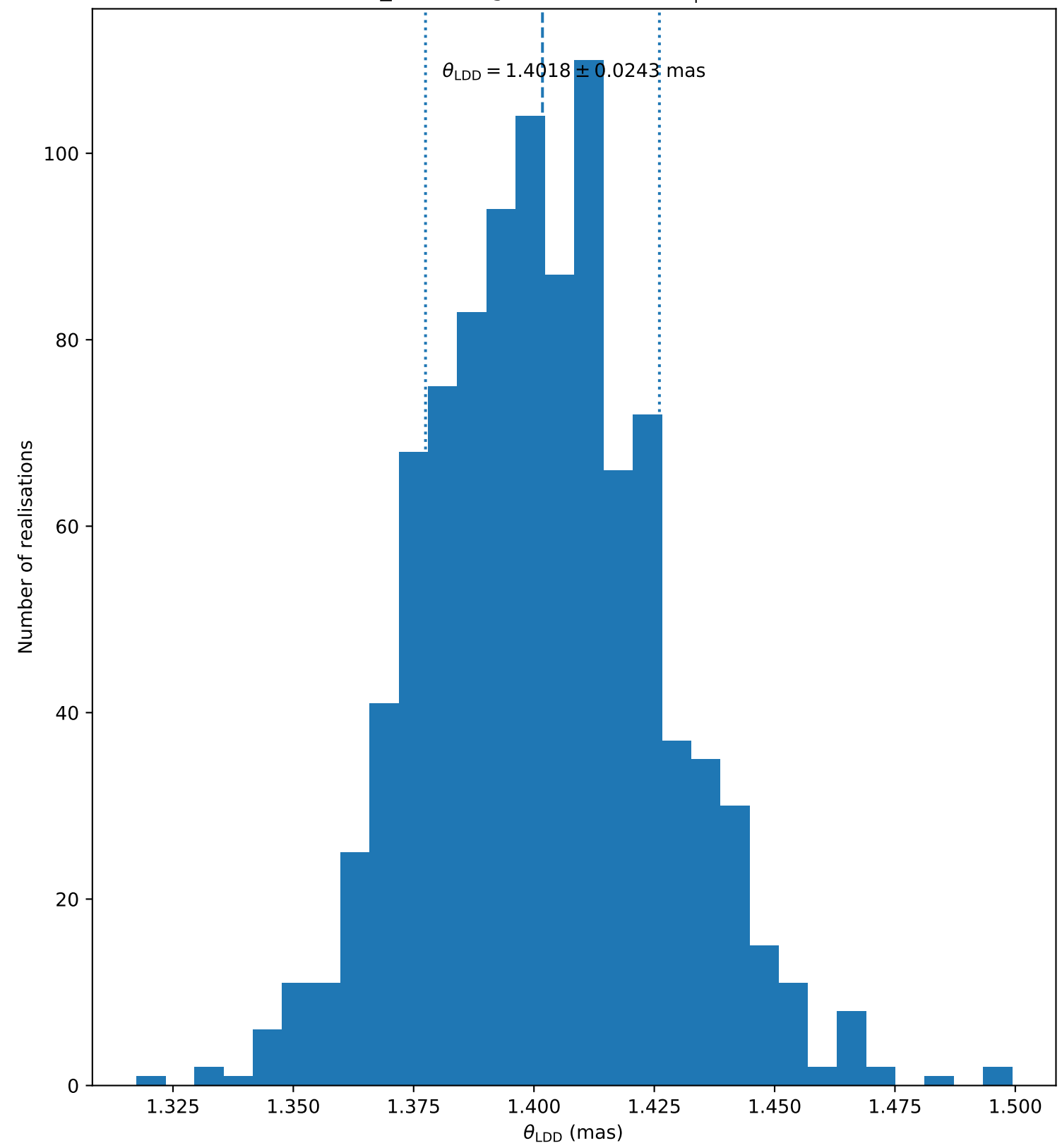
ksi_Gem (bright, 106) ( N_{\text{bootstrap}} = 1000 )
