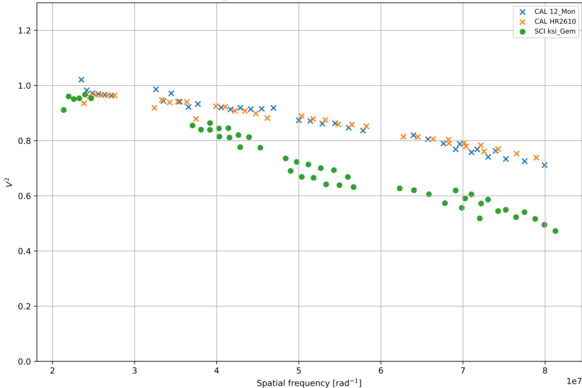
ksi_Gem - complete calibrated sequence
