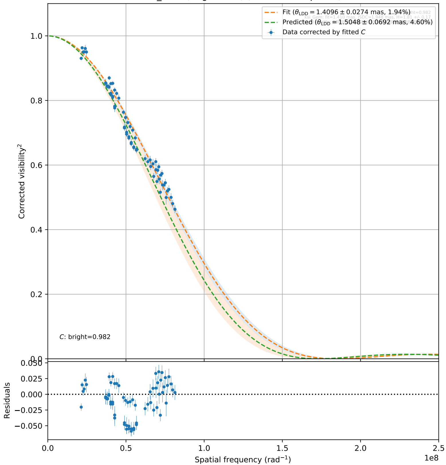
ksi_Gem (bright, 106) (66 valid vis 2 points)
