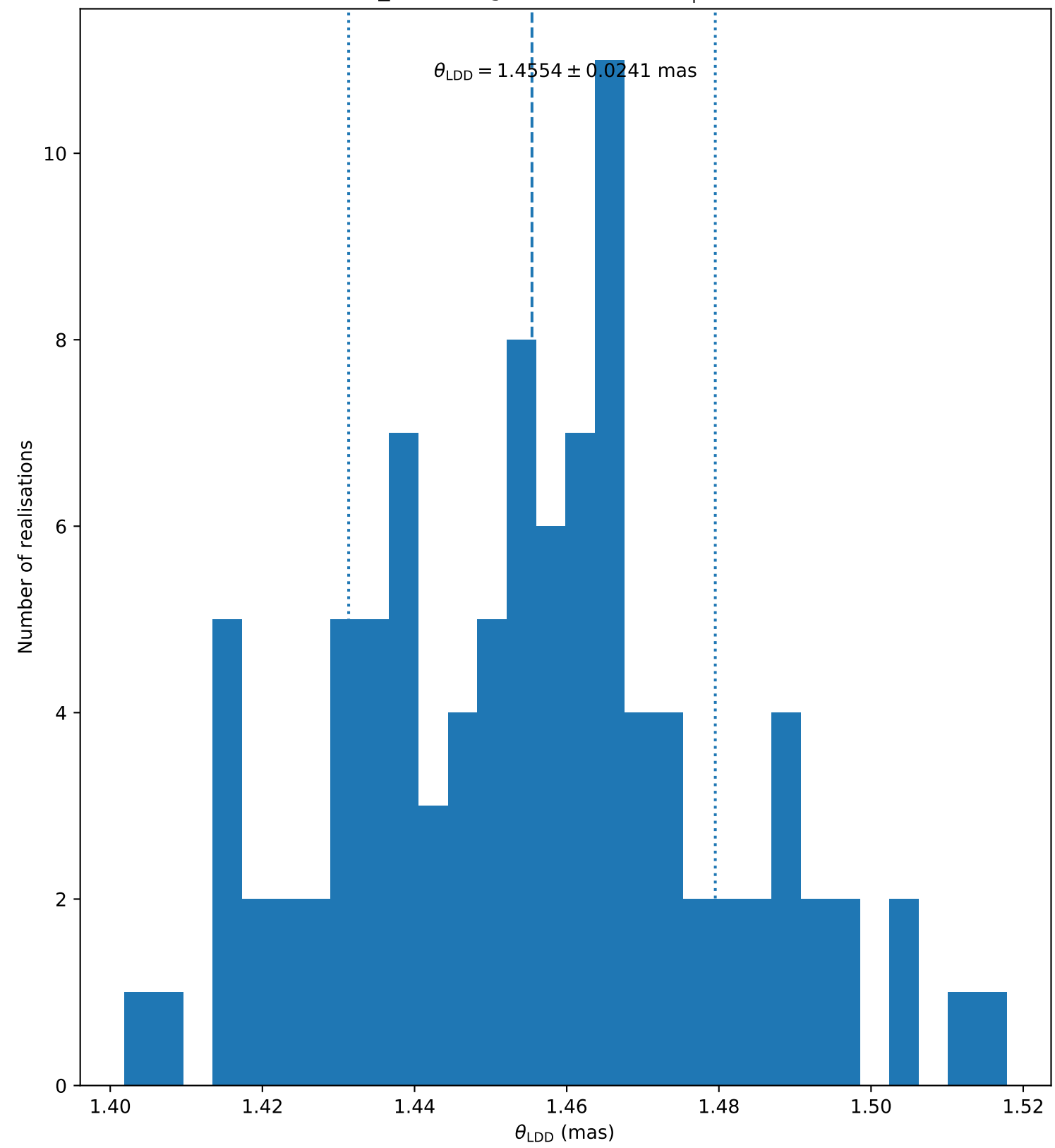
ksi_Gem (bright, 106) ( N_{\text{bootstrap}} = 100 )
