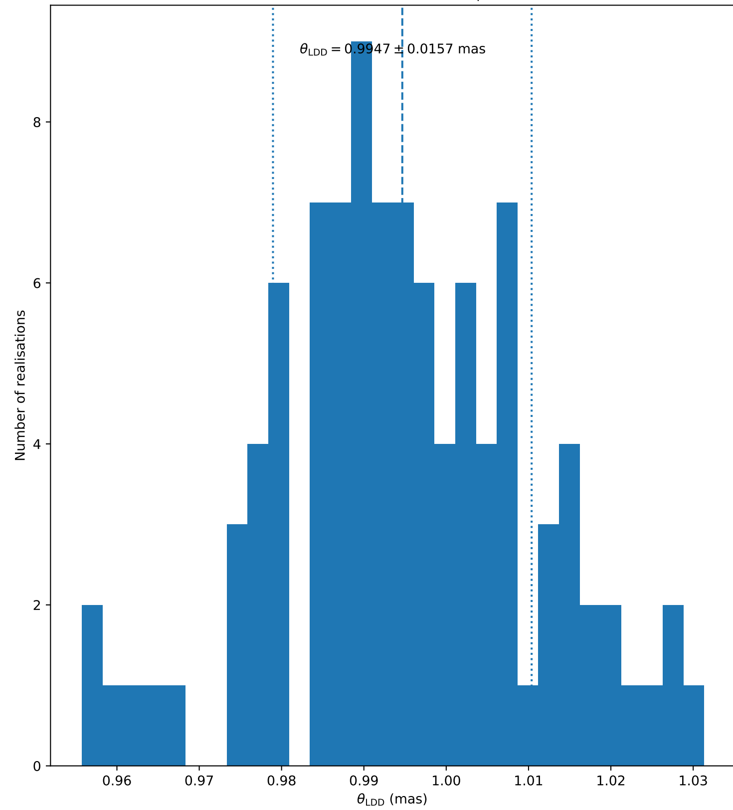
ksi_Gem (faint, 106) ( N_{\text{bootstrap}} = 100 )
