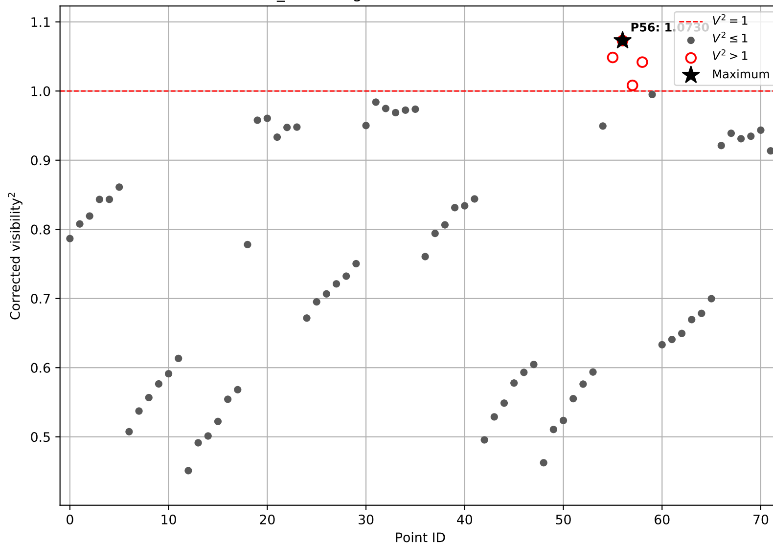
ksi_Gem, bright, 106: corrected V2 values
