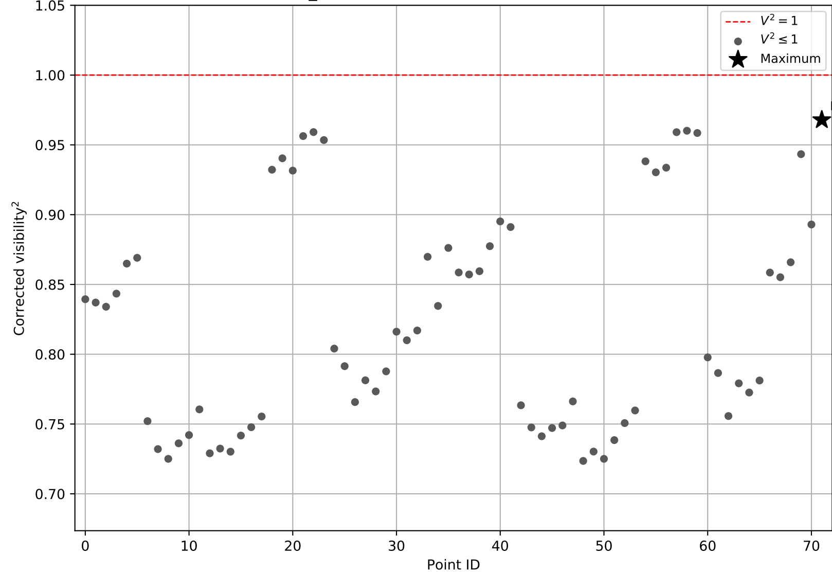
ksi_Gem, faint, 106: corrected V2 values
