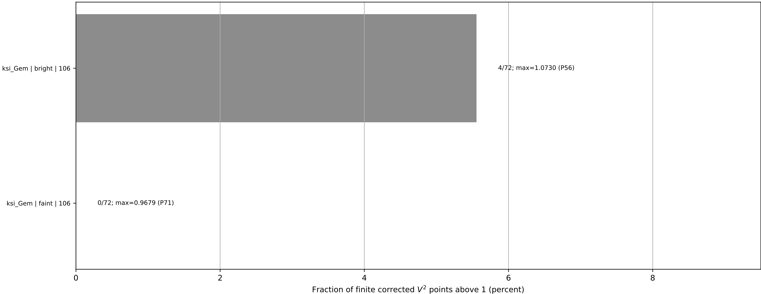
Corrected V^2 > 1 overview Labels show N(V^2 > 1)/N(\text{total}) , maximum V^2 and maximum point
