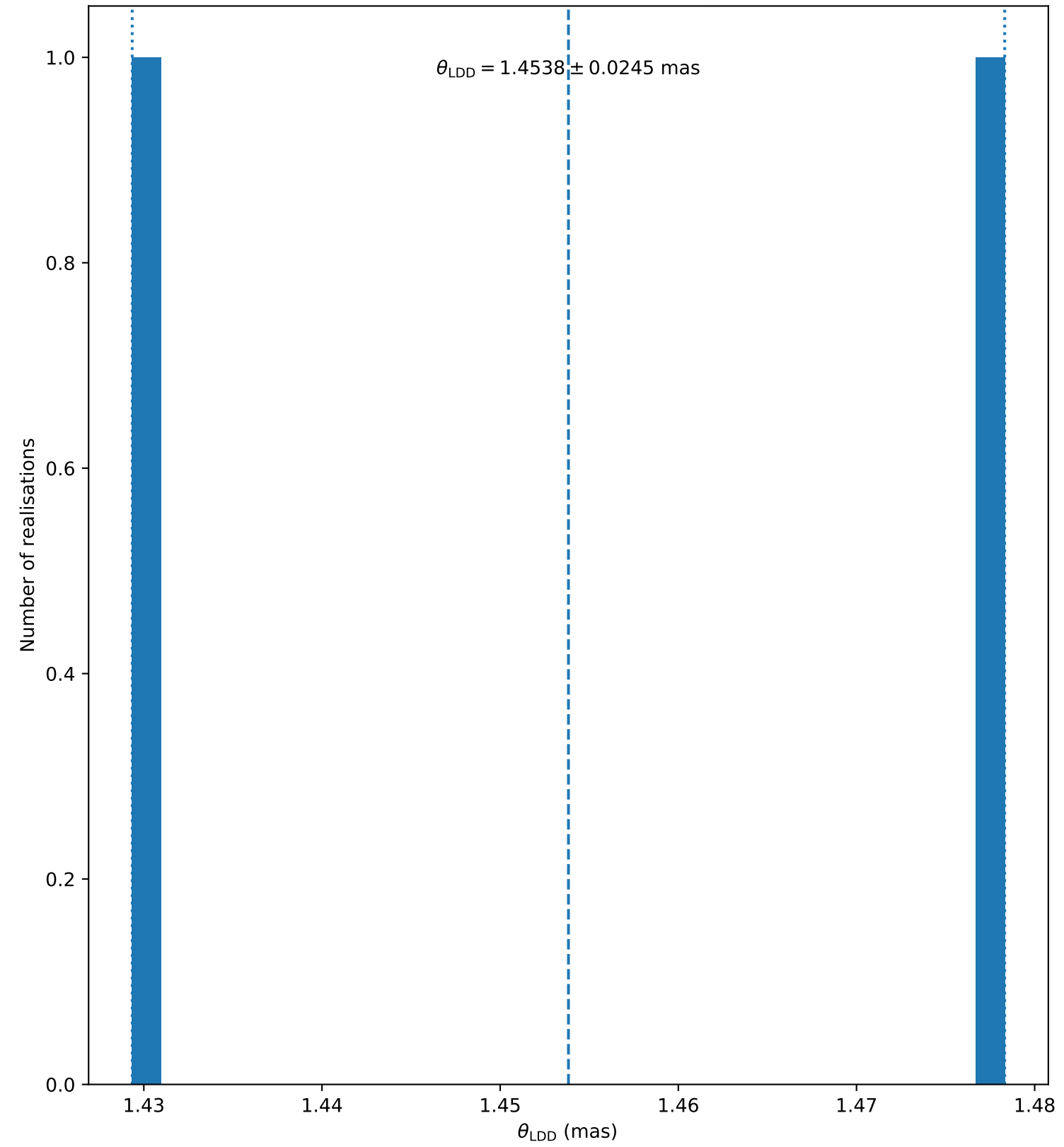
ksi_Gem (bright, 106) ( N_{\text{bootstrap}} = 2 )
