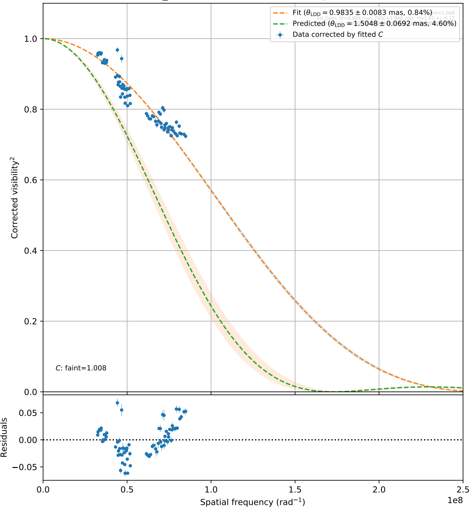
ksi_Gem (faint, 106) (72 valid vis 2 points)
