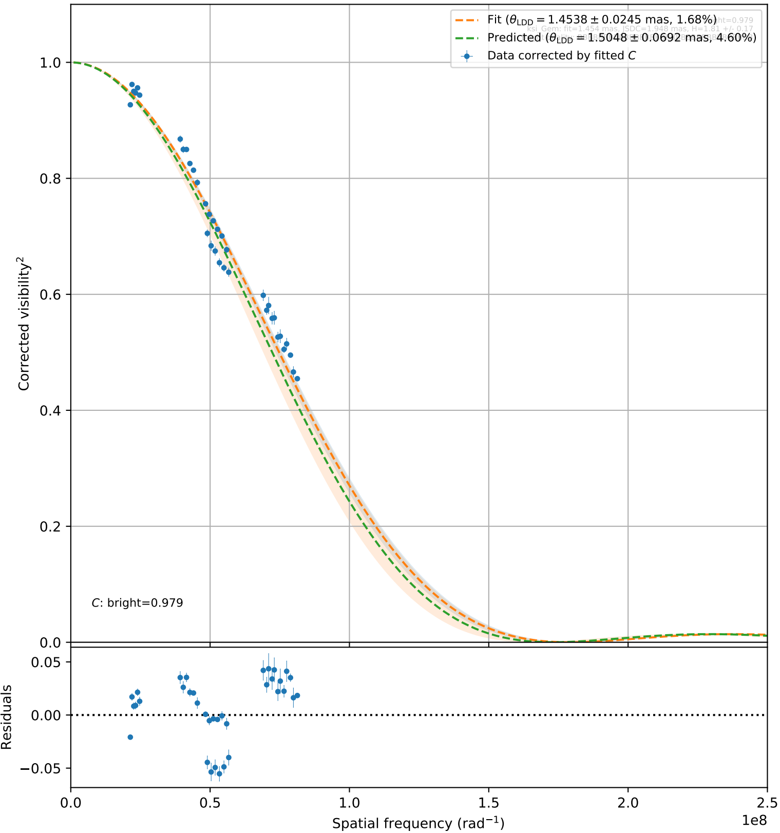
ksi_Gem (bright, 106) (36 valid vis 2 points)
