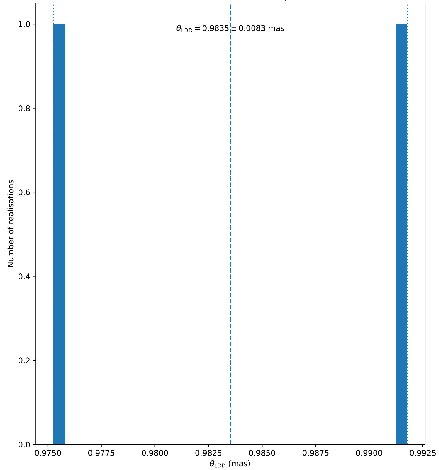
ksi_Gem (faint, 106) ( N_{\text{bootstrap}} = 2 )
