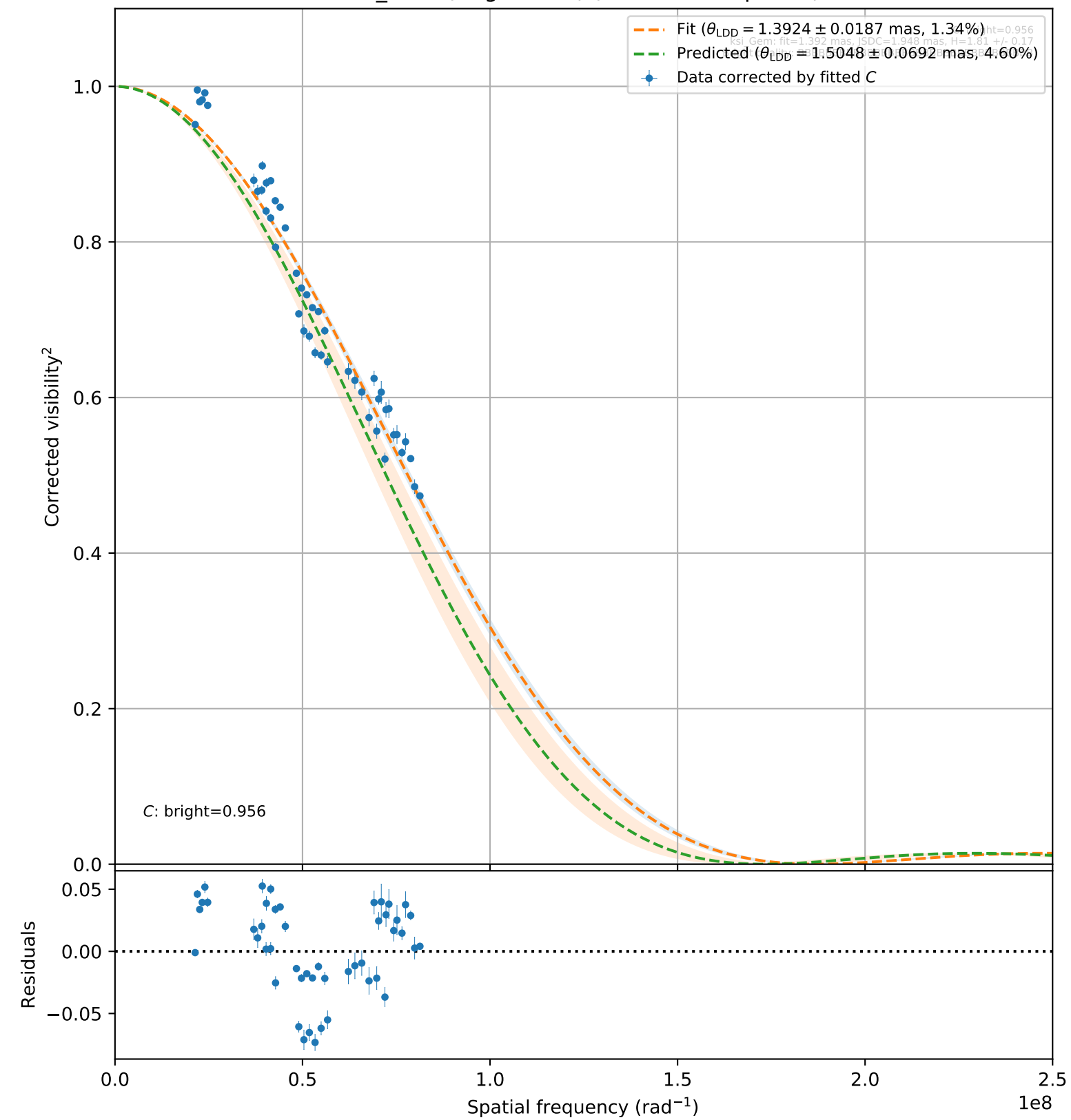
ksi_Gem (bright, 106) (48 valid vis 2 points)
