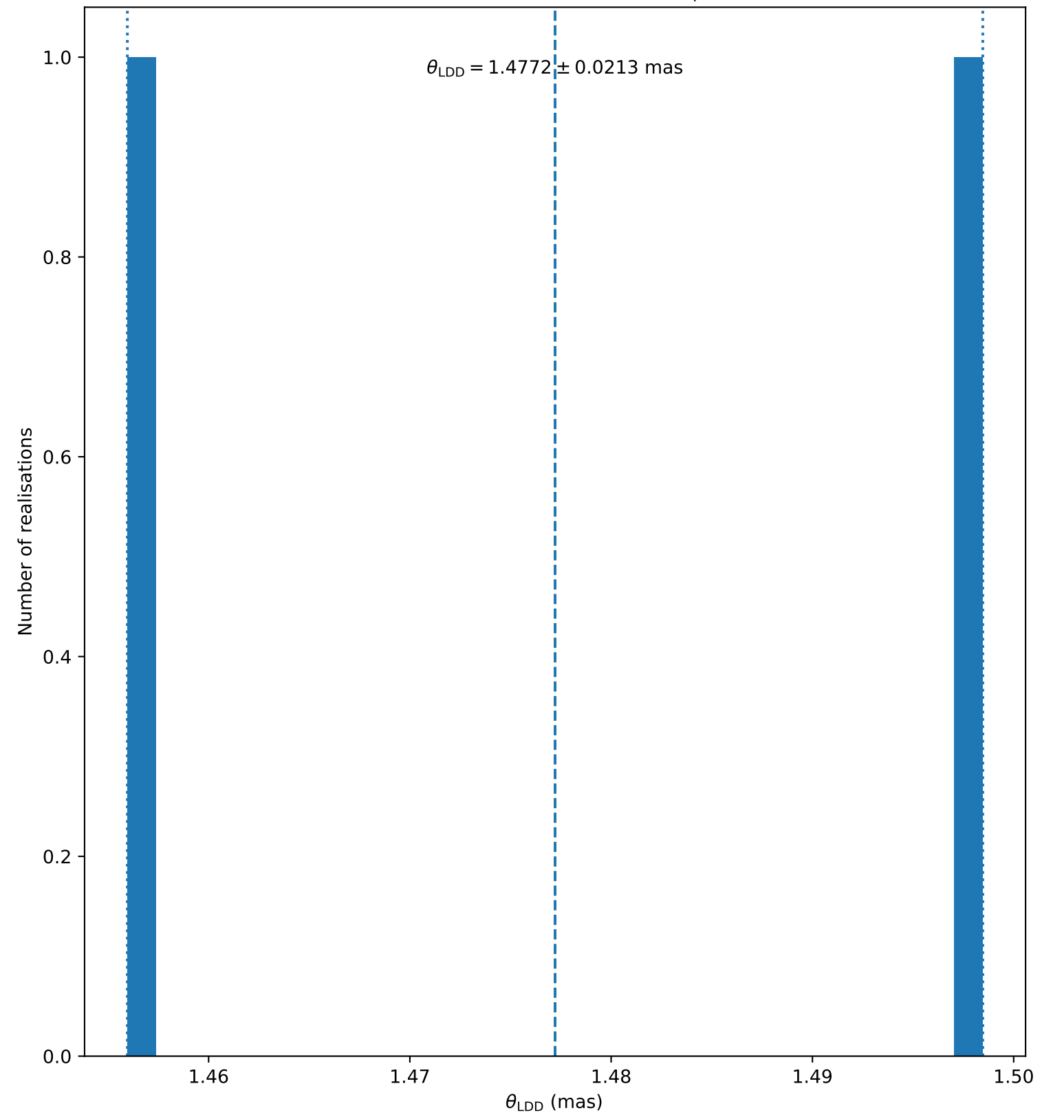
ksi_Gem (bright, 106) ( N_{\text{bootstrap}} = 2 )
