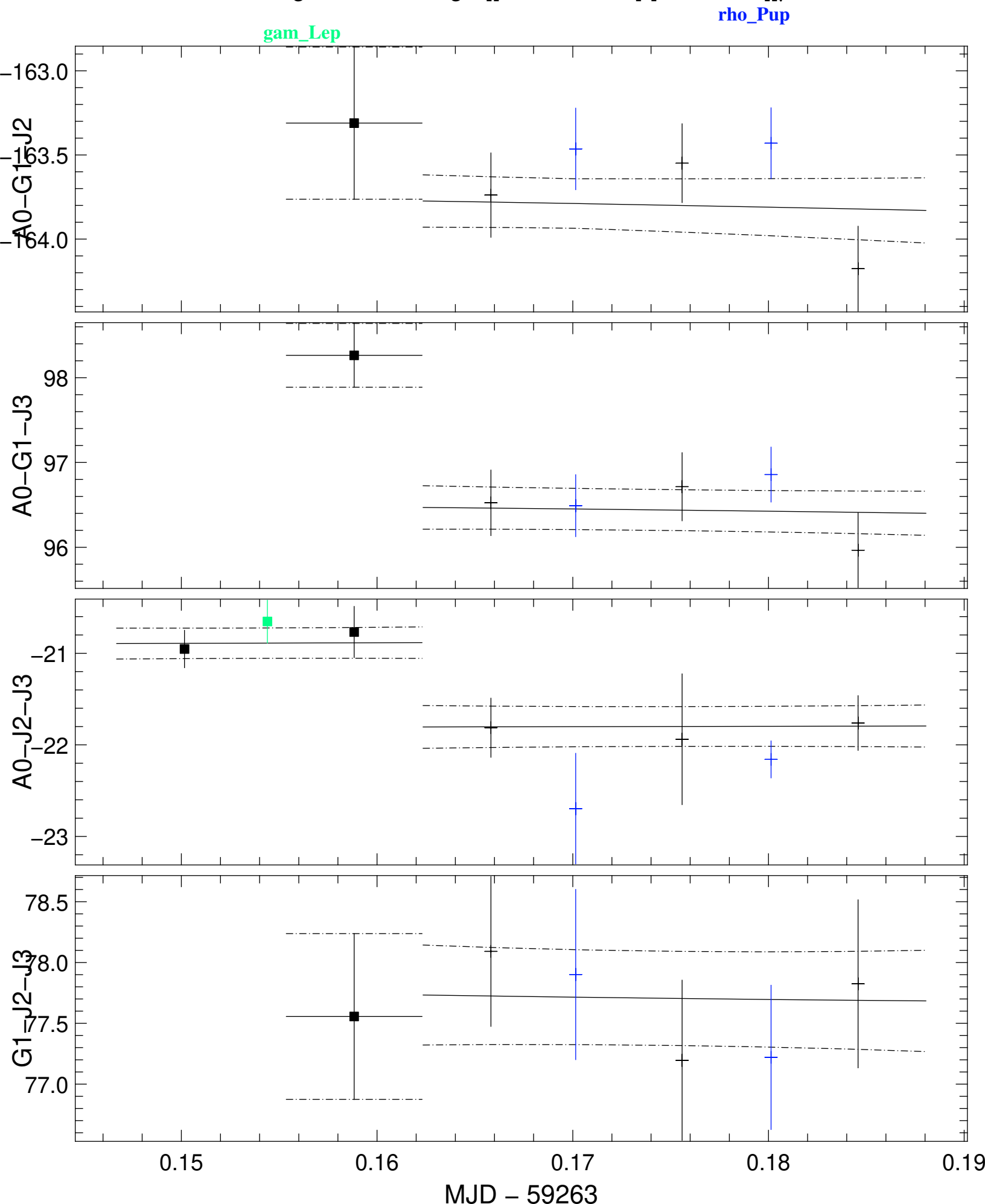
Transfer-Function t3Phi (black) and Scientific t3Phi (colors) averaged in the range [[1.637,1.715],[2.04,2.25]]\mu\text{m}
