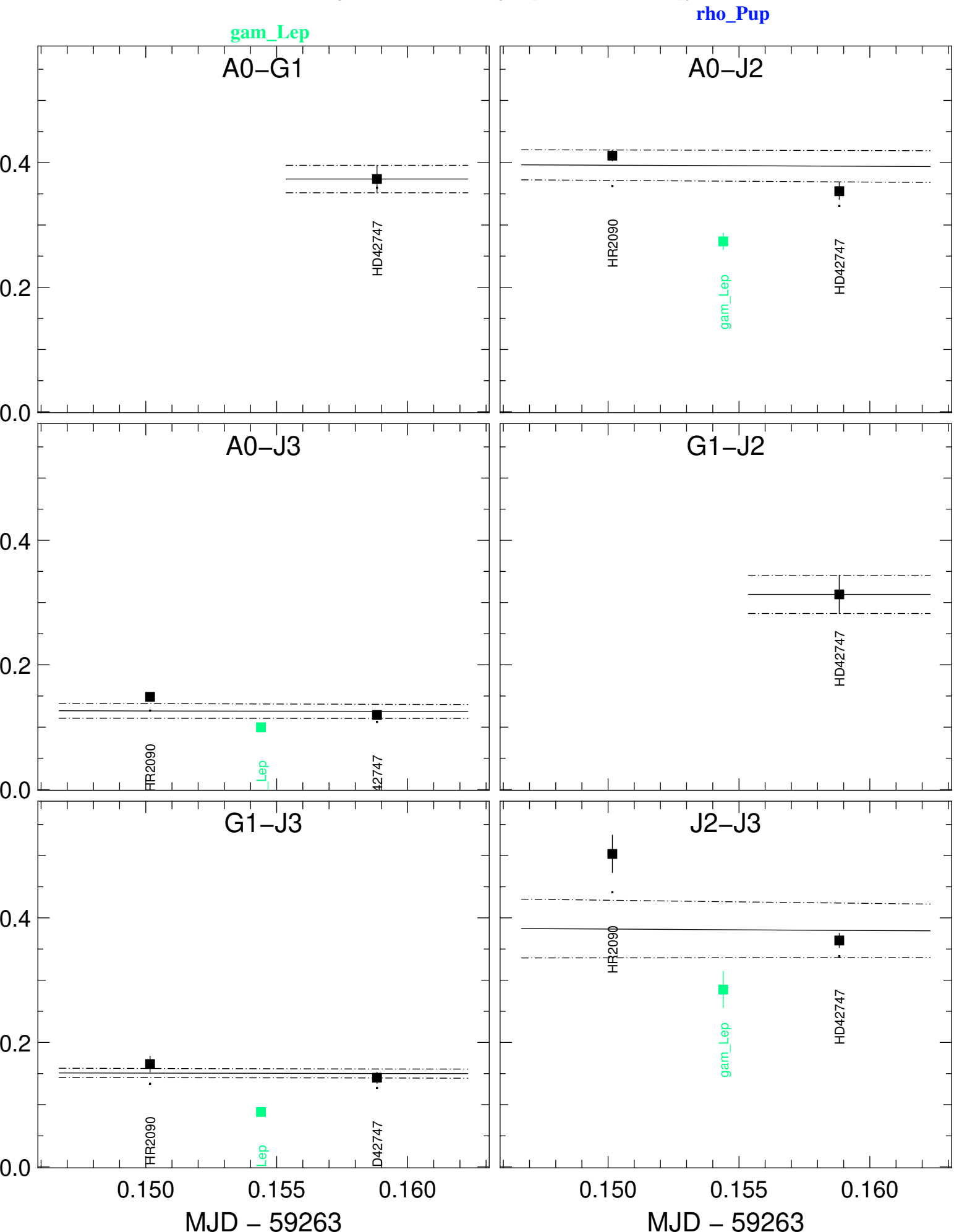
Transfer-Function vis2 (black) and Scientific vis2 (colors) averaged in the range [1.725,1.725] \mu m
