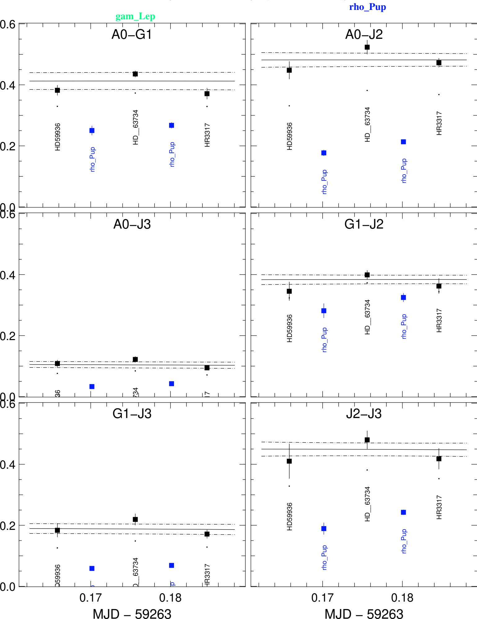
Transfer-Function vis2 (black) and Scientific vis2 (colors) averaged in the range [1.677,1.677] \mu m
