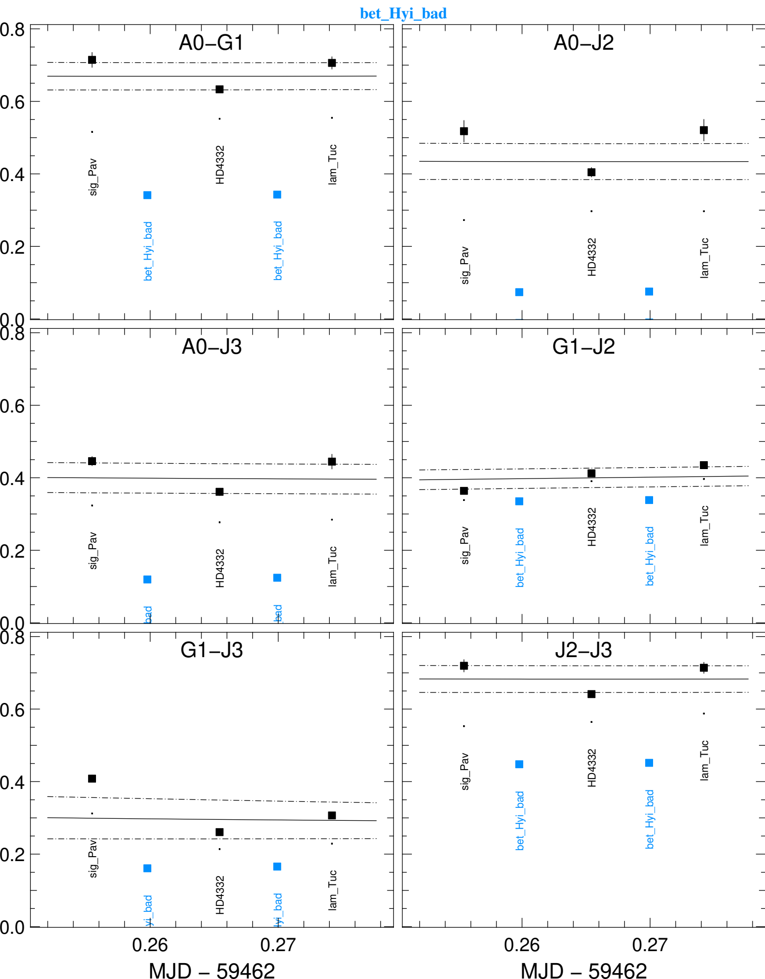
Transfer-Function vis2 (black) and Scientific vis2 (colors) averaged in the range [1.773,1.773] \mu m
