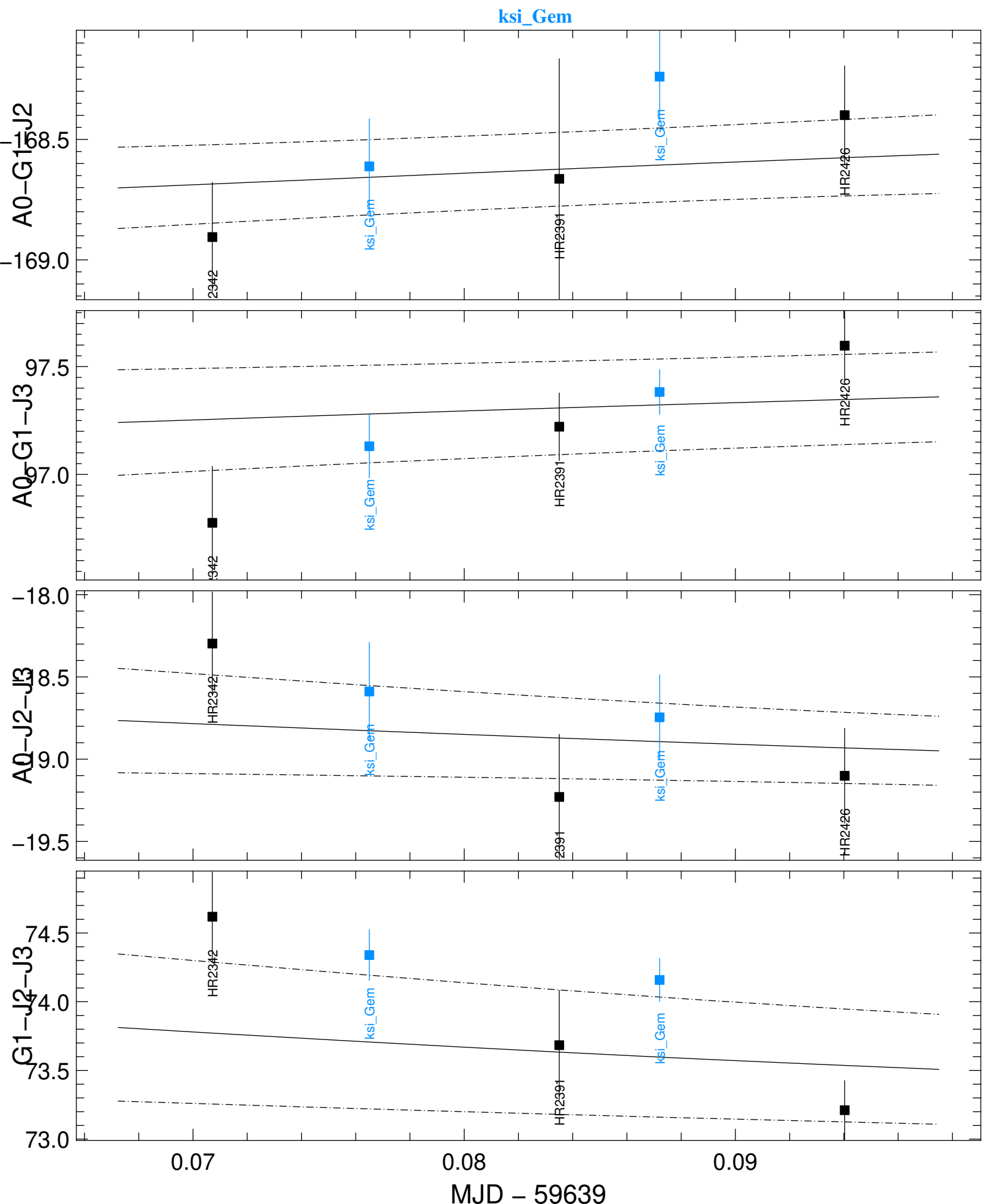
Transfer-Function t3Phi (black) and Scientific t3Phi (colors) averaged in the range [1.725,1.725] \mu m
