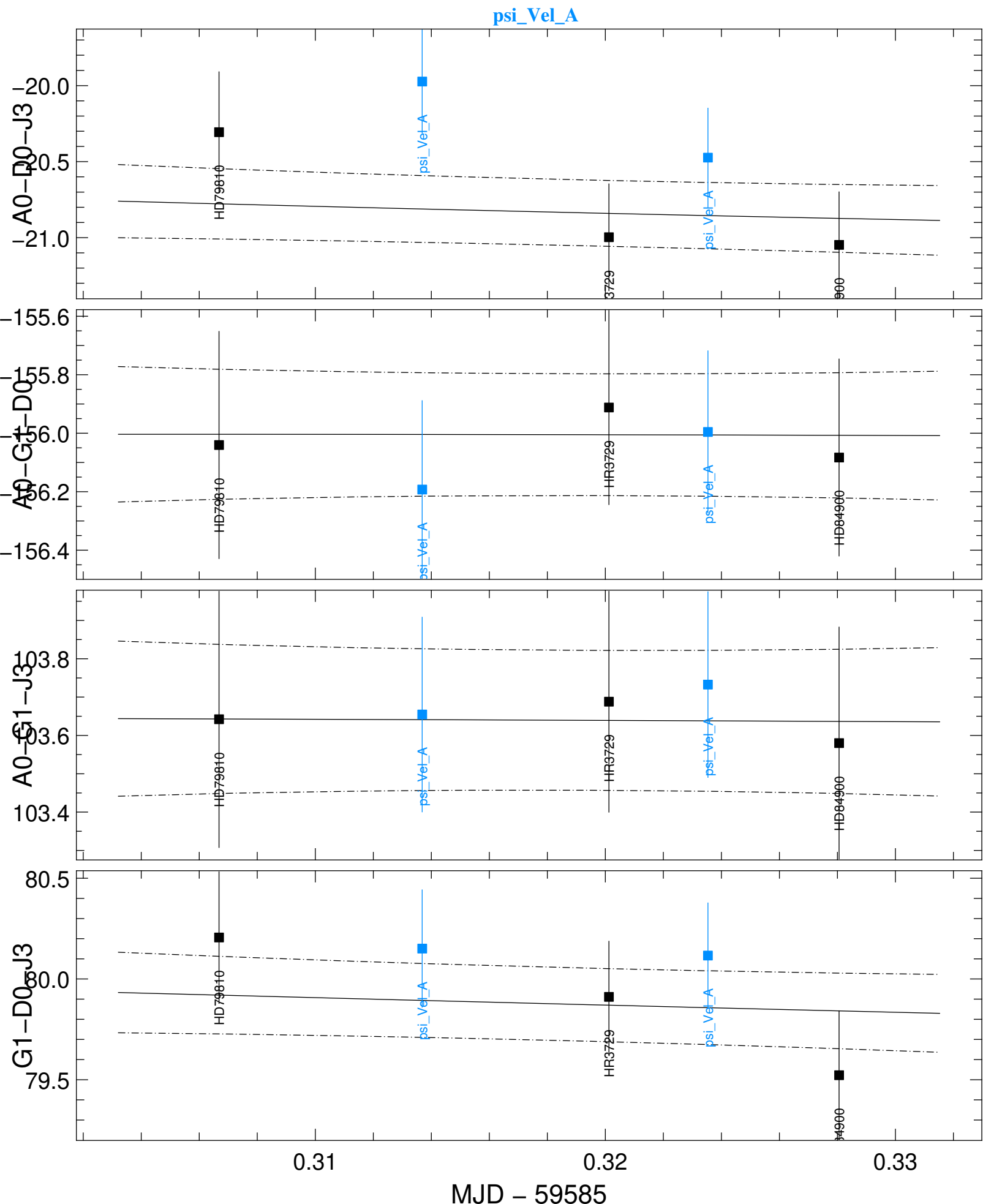
Transfer-Function t3Phi (black) and Scientific t3Phi (colors) averaged in the range [1.581, 1.581]\mu\text{m}
