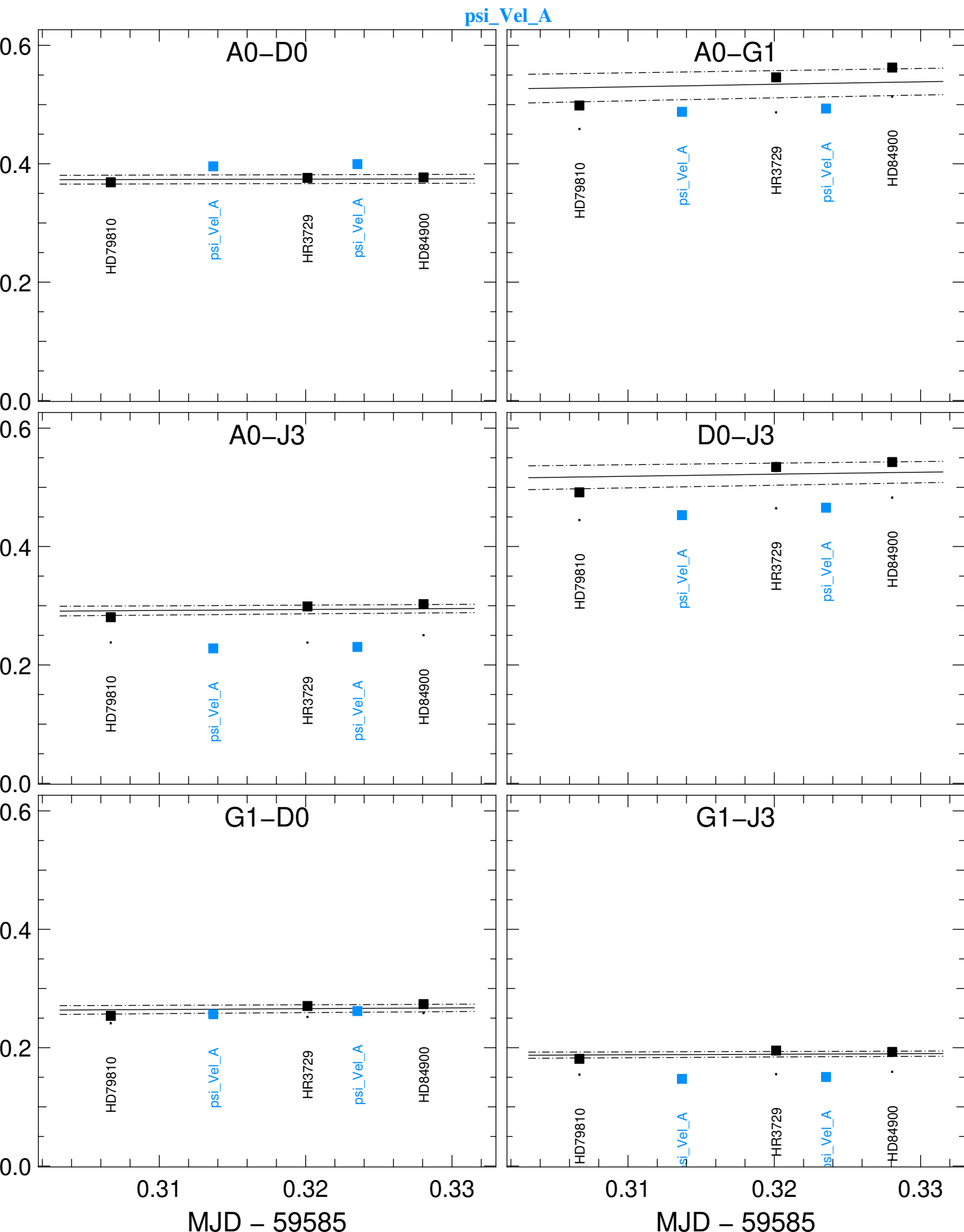
Transfer-Function vis2 (black) and Scientific vis2 (colors) averaged in the range [1.629, 1.629]\mu\text{m}
