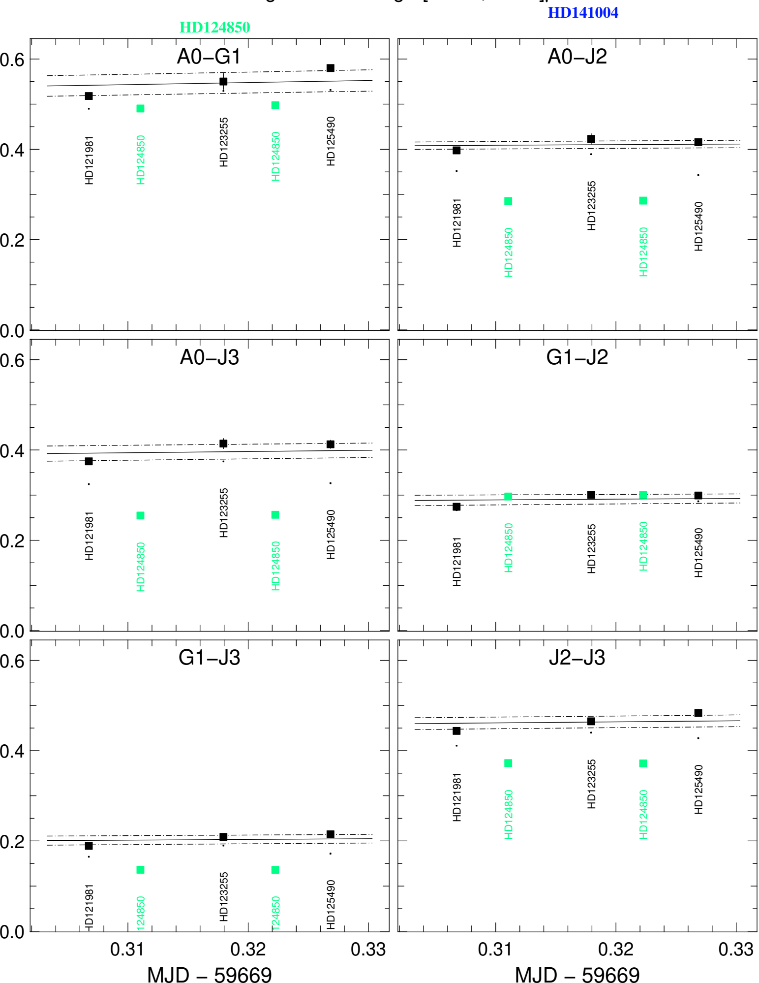
Transfer-Function vis2 (black) and Scientific vis2 (colors) averaged in the range [1.533, 1.533]\mu\text{m}
