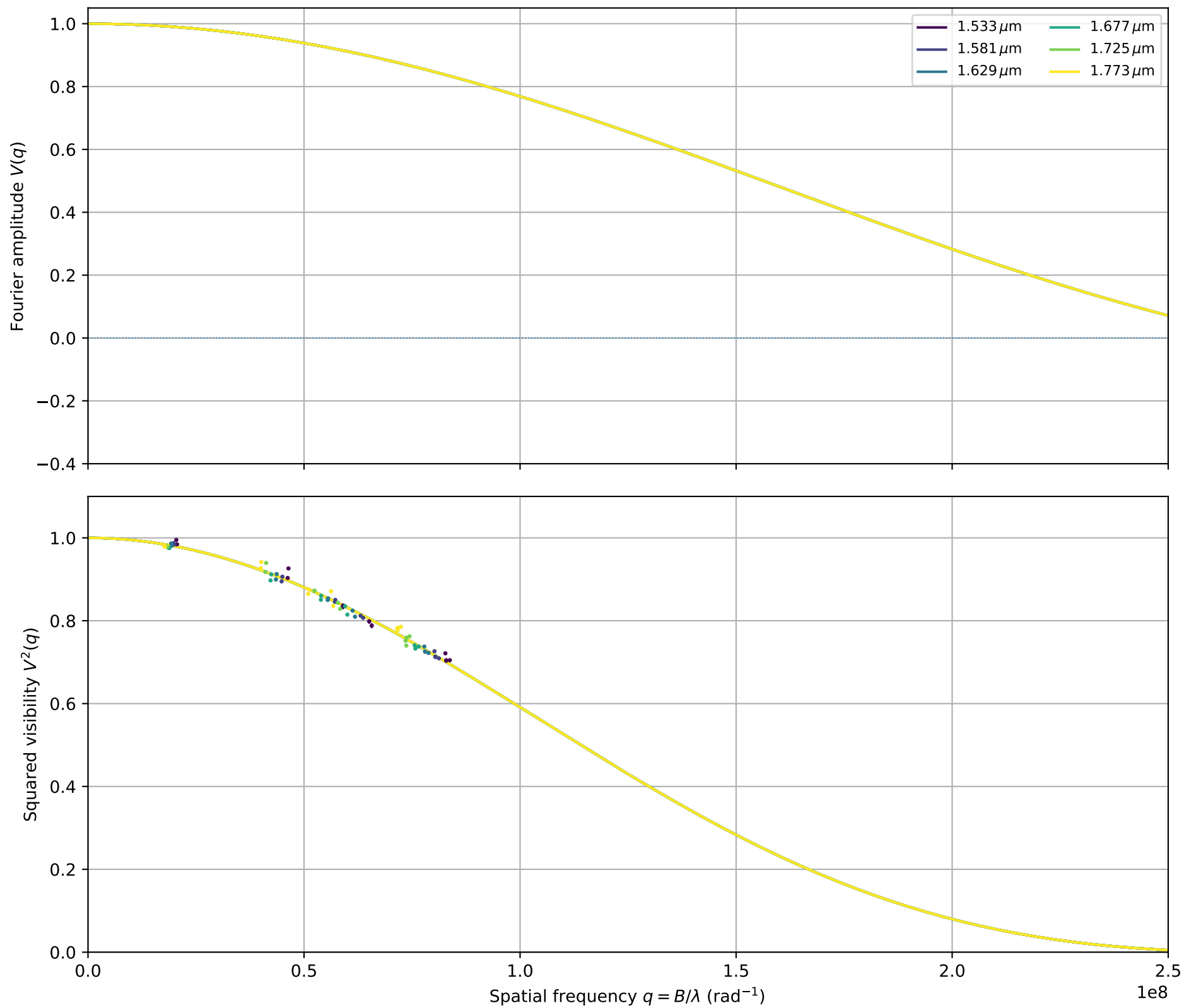
psi Vel A: fitted \theta_{\text{LDD}} = 0.9455 \pm 0.0043 mas
