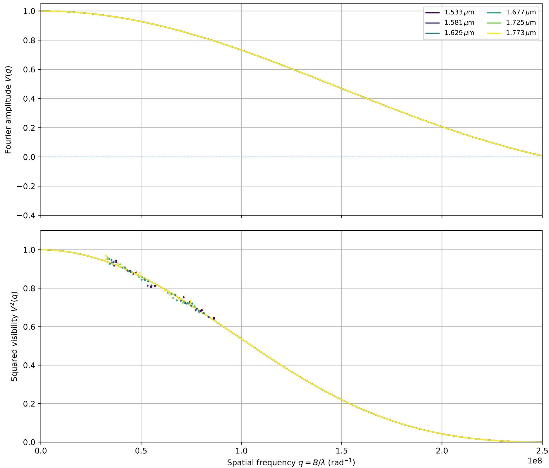
HR_2998: fitted \theta_{\text{LDD}} = 1.0375 \pm 0.0063 mas
