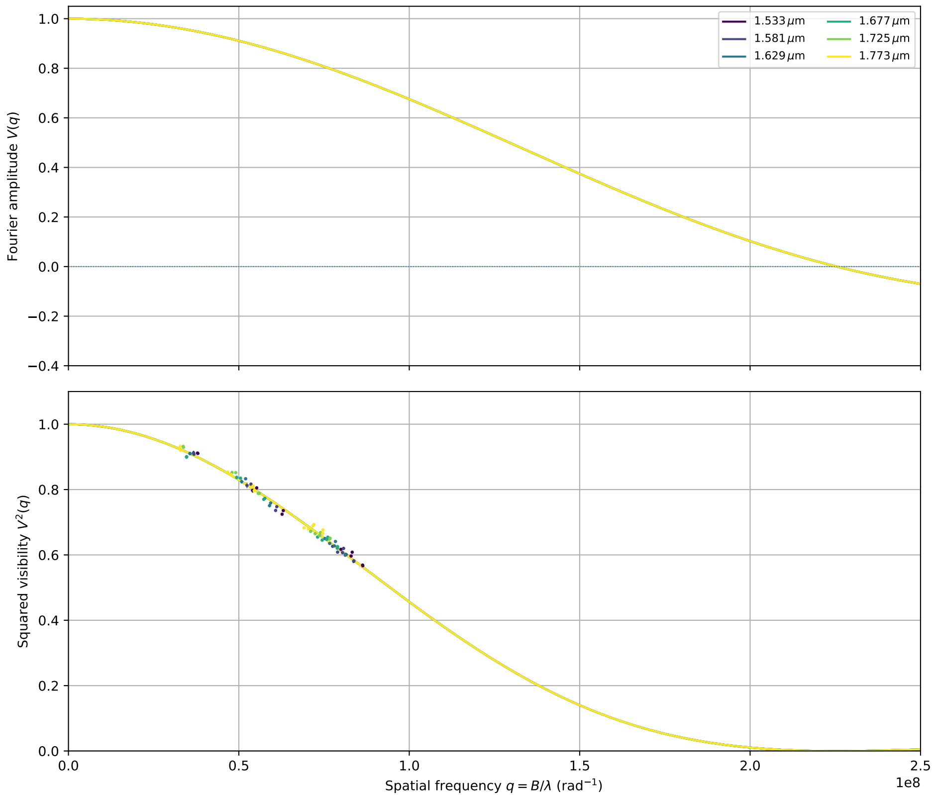
HD124850: fitted \theta_{\text{LDD}} = 1.1446 \pm 0.0073 mas
