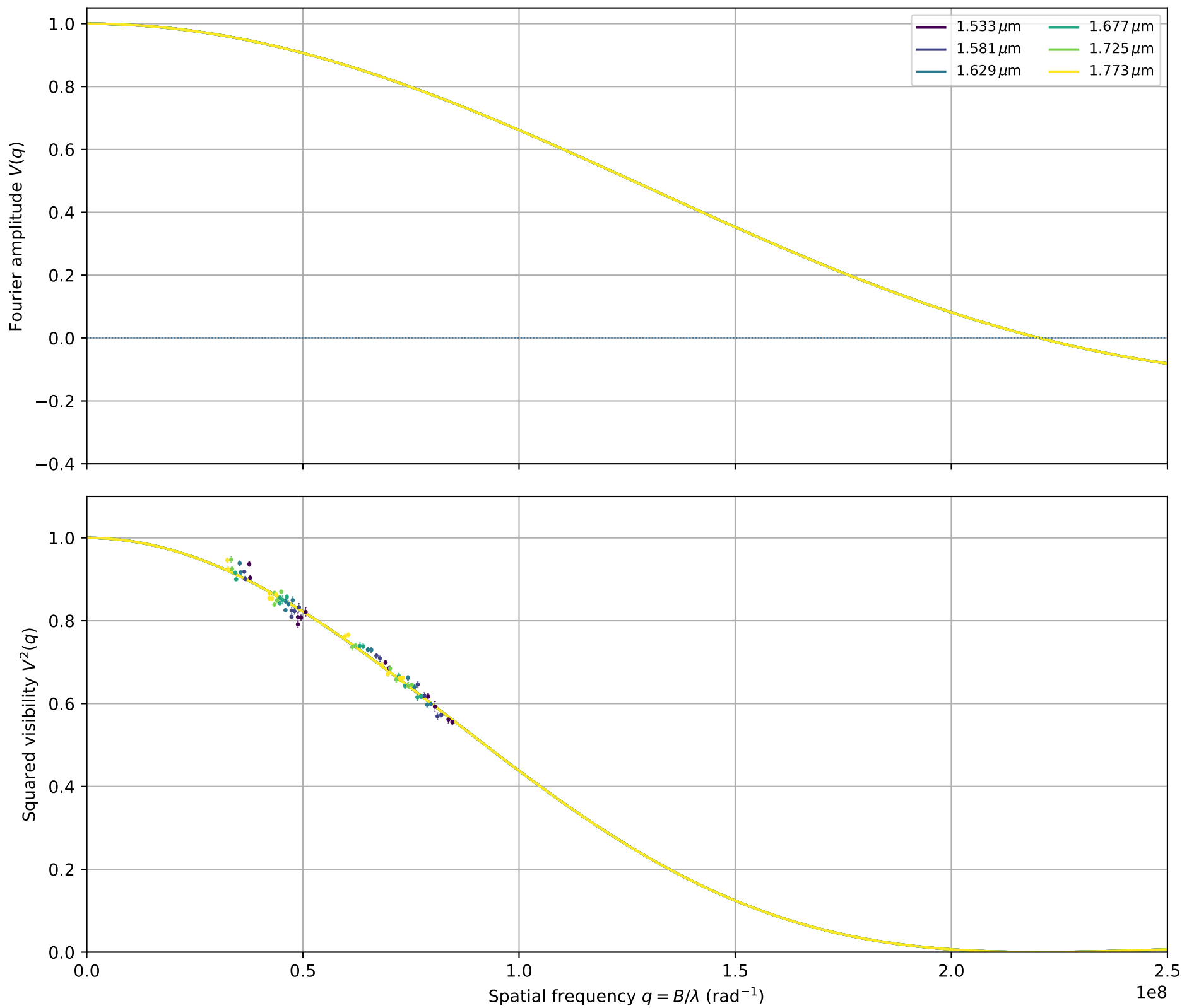
HD142860: fitted \theta_{\text{LDD}} = 1.1747 \pm 0.0089 mas
