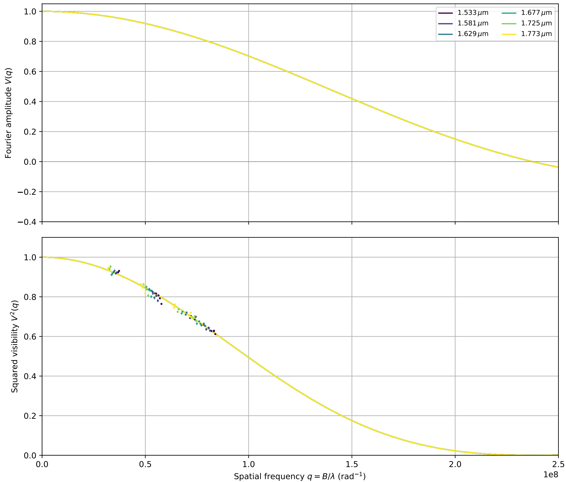
HD141004: fitted \theta_{\text{LDD}} = 1.0940 \pm 0.0069 mas
