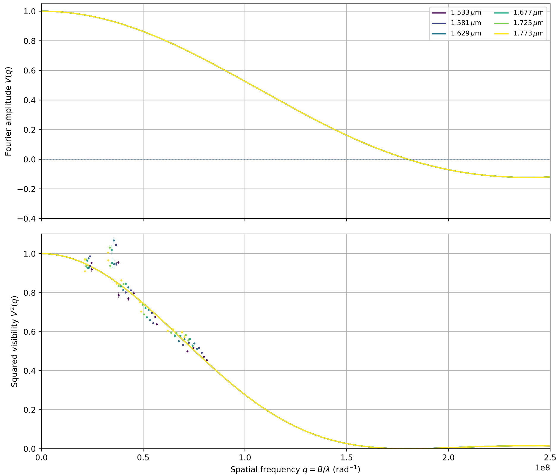
ksi_Gem: fitted \theta_{\text{LDD}} = 1.4315 \pm 0.0084 mas
