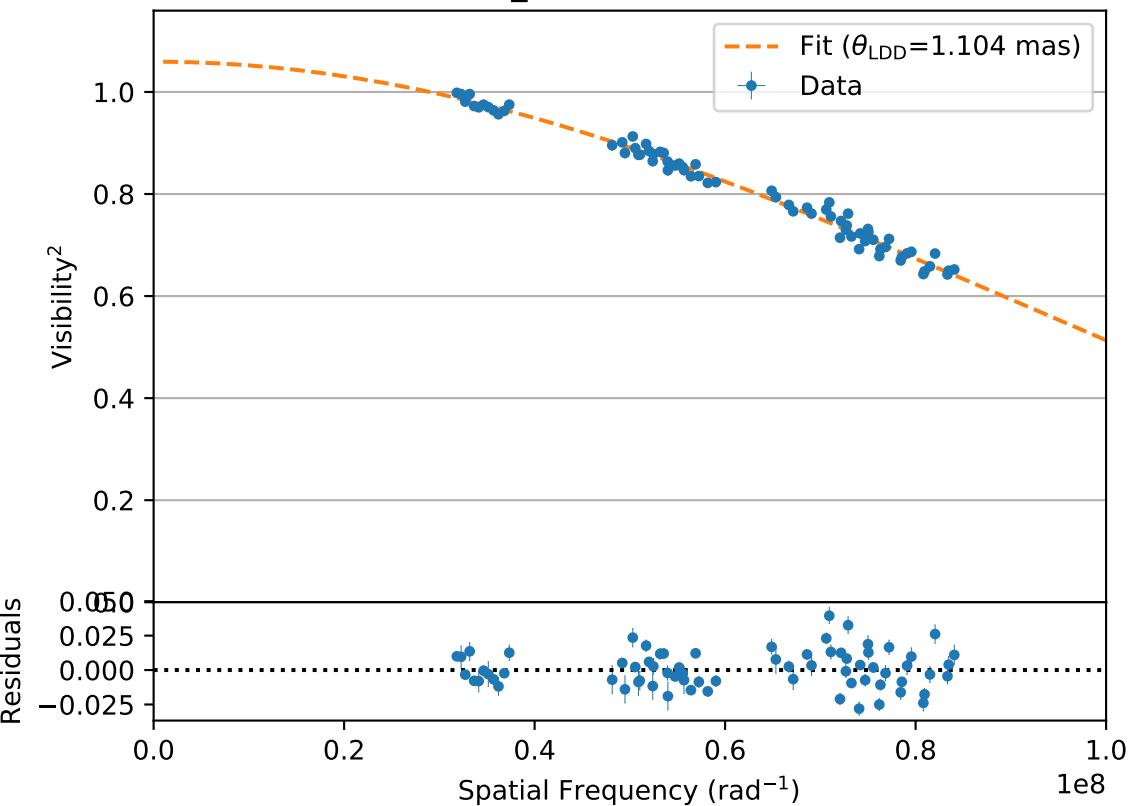
iot_Psc (faint, P104)
