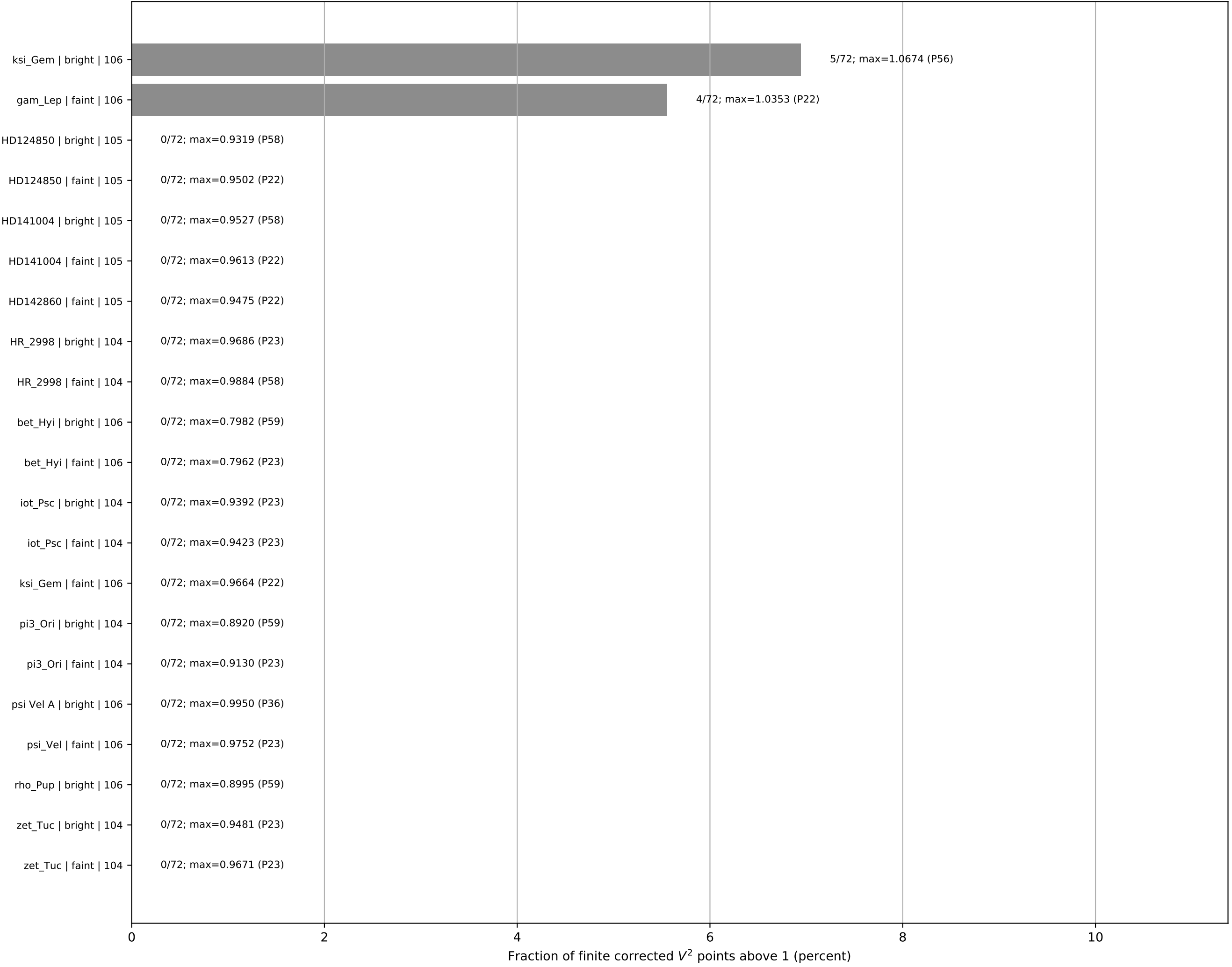
Corrected V2 > 1 overview Labels show N(V2 > 1)/N(total), maximum V2 and maximum point
