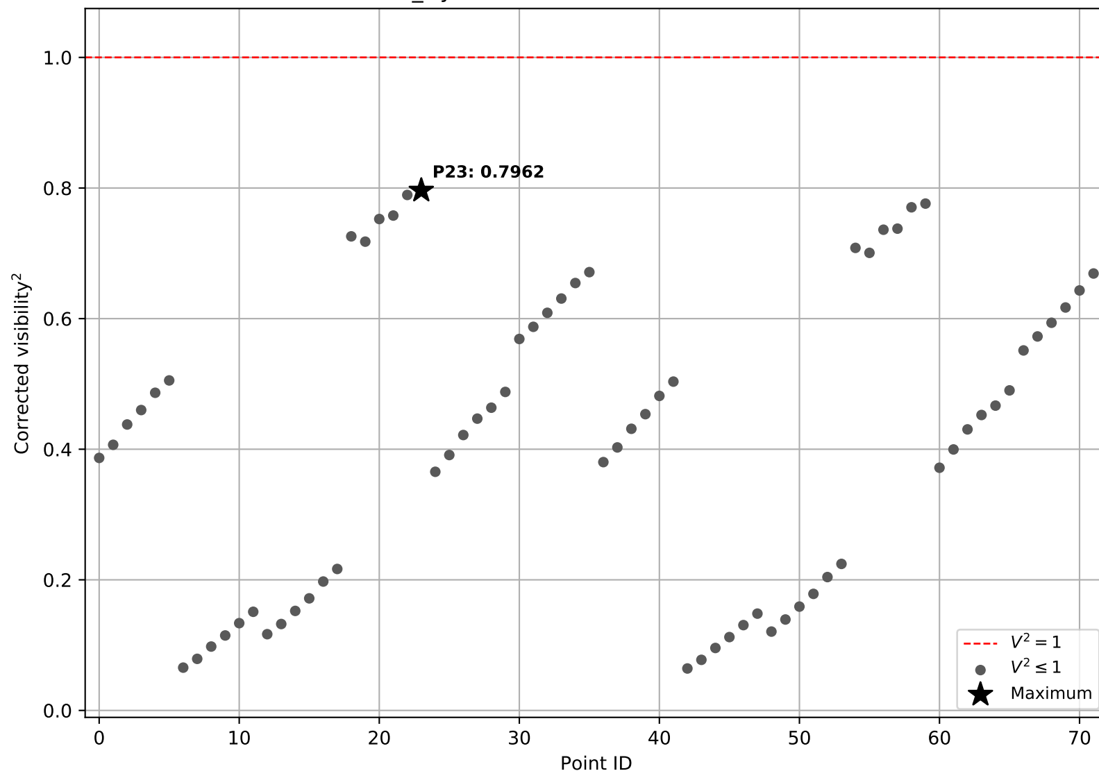
bet_Hyi, faint, 106: corrected V2 values
