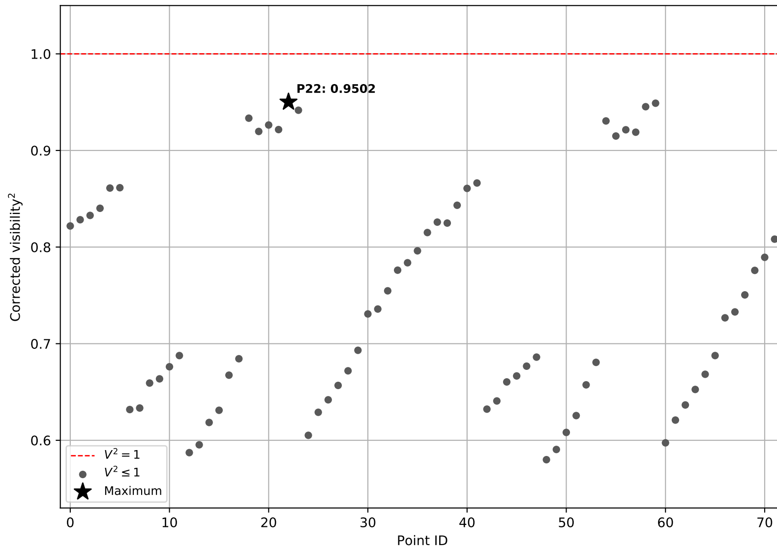
HD124850, faint, 105: corrected V2 values
