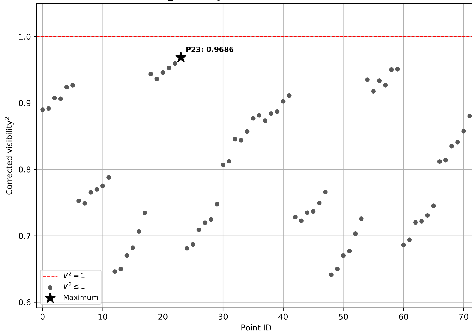
HR_2998, bright, 104: corrected V2 values
