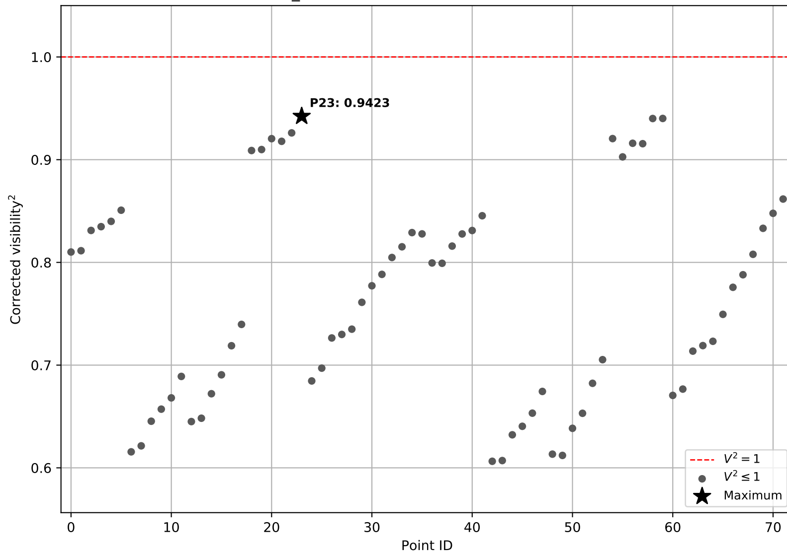
iot_Psc, faint, 104: corrected V2 values
