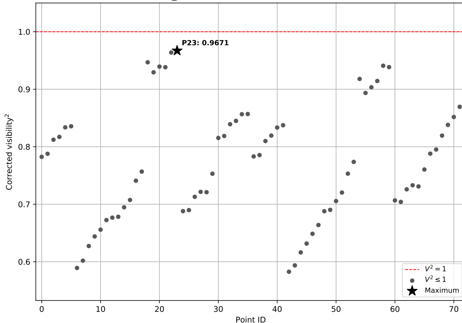
zet_Tuc, faint, 104: corrected V2 values
