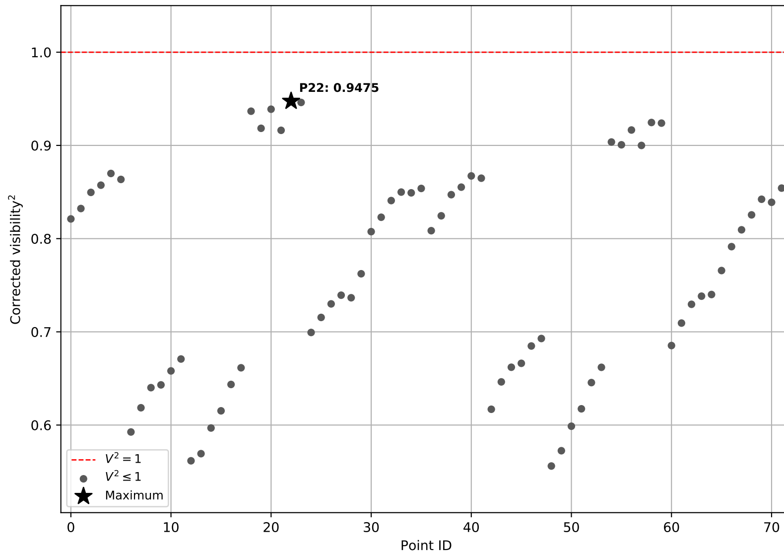
HD142860, faint, 105: corrected V2 values
