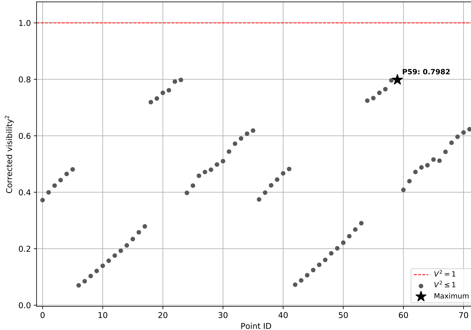
bet_Hyi, bright, 106: corrected V2 values
