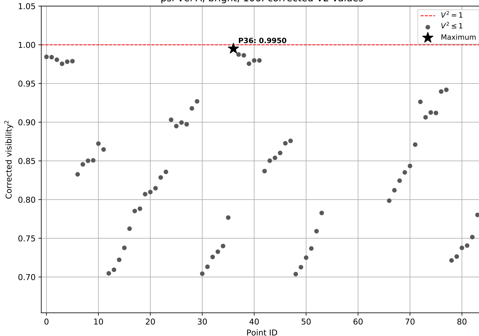
psi Vel A, bright, 106: corrected V2 values
