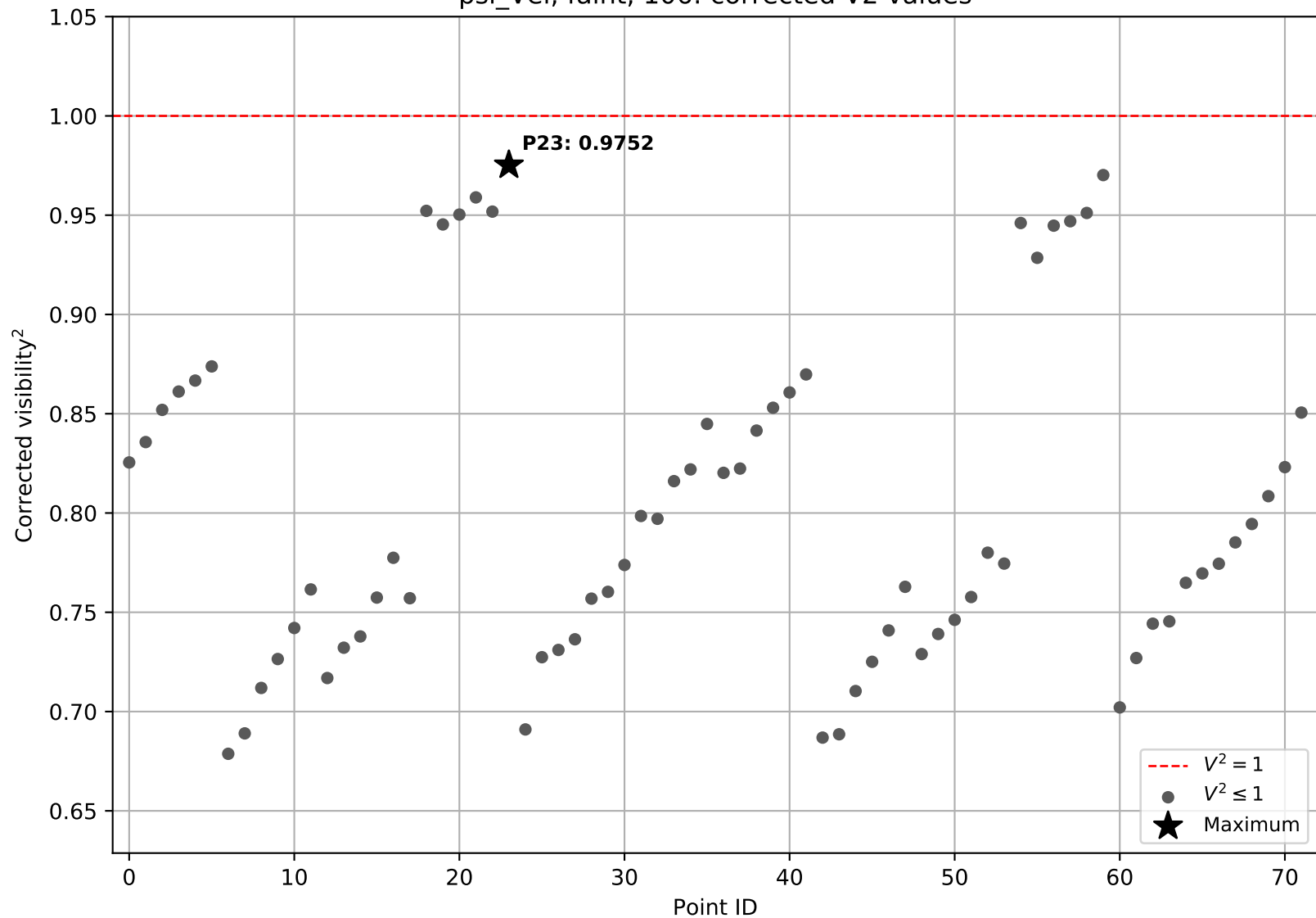
psi_Vel, faint, 106: corrected V2 values
