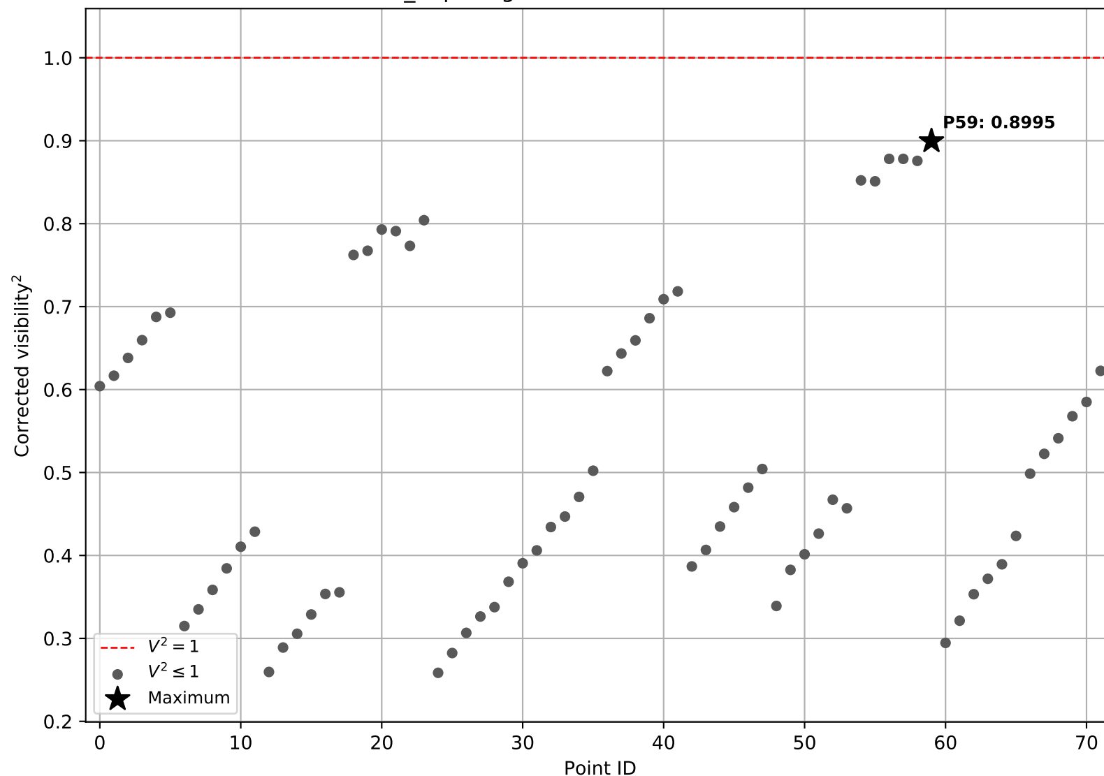
rho_Pup, bright, 106: corrected V2 values
