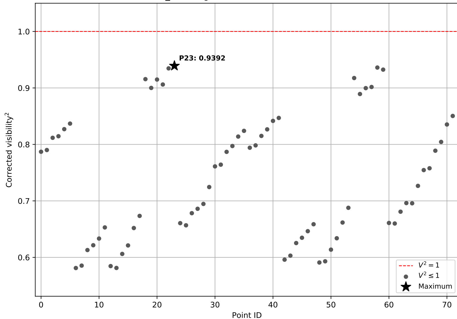
iot_Psc, bright, 104: corrected V2 values
