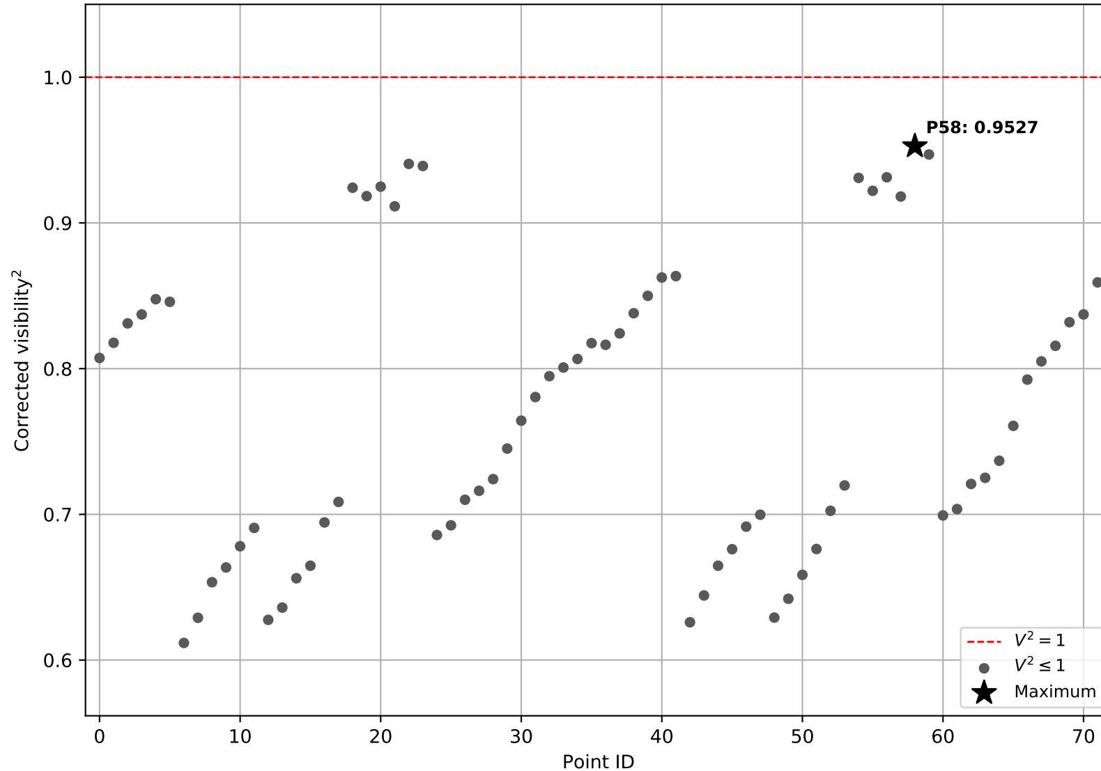
HD141004, bright, 105: corrected V2 values
