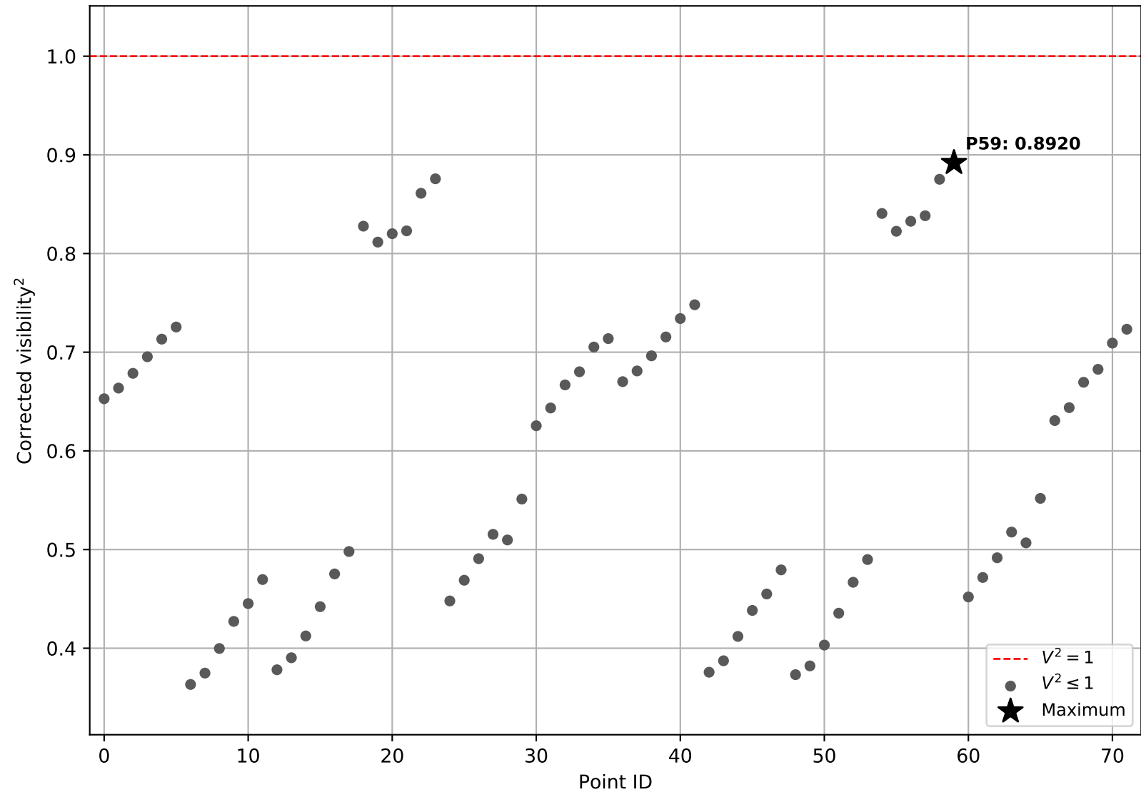
pi3_Ori, bright, 104: corrected V2 values
