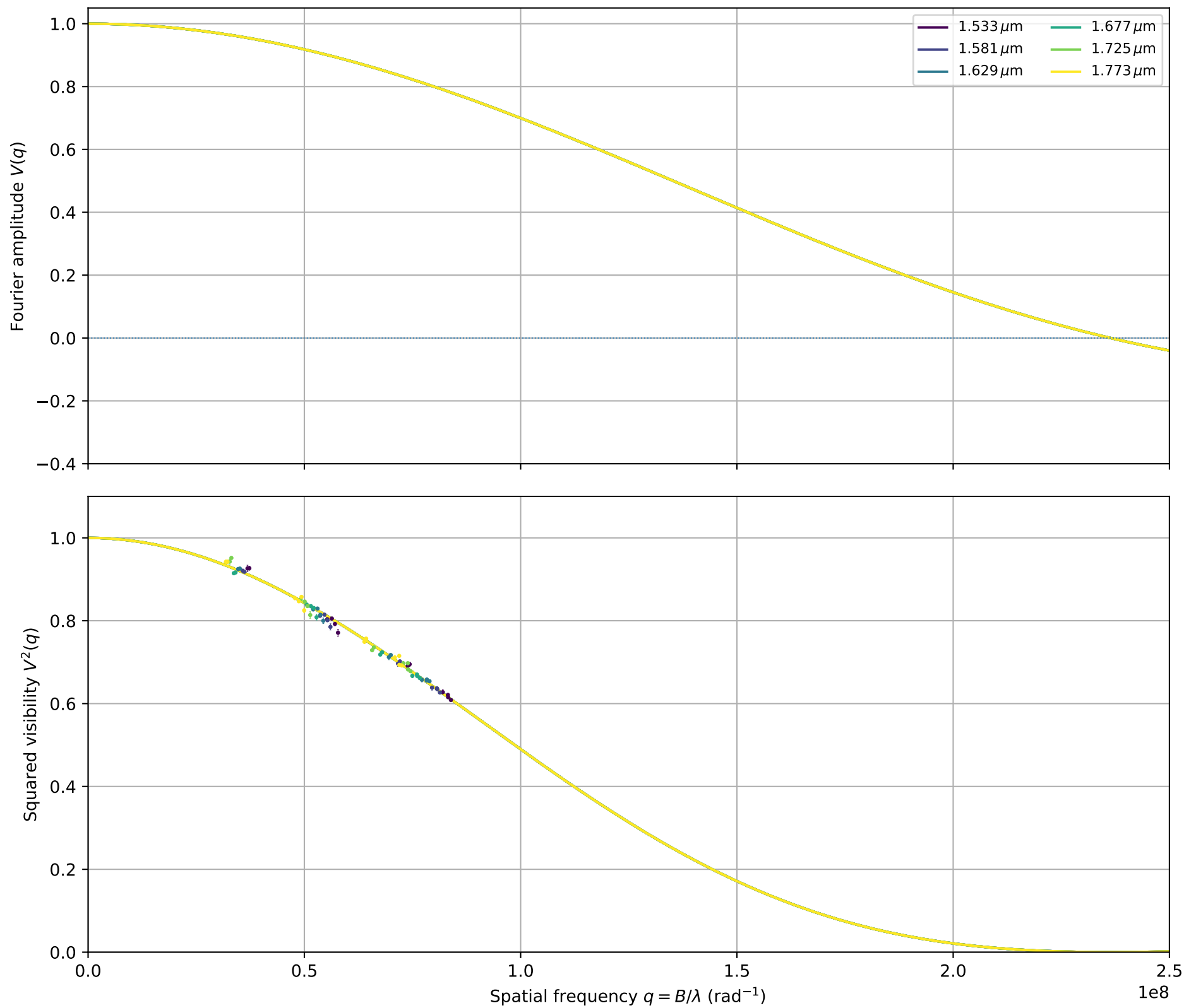
HD141004: fitted \theta_{\text{LDD}} = 1.1028 \pm 0.0018 mas
