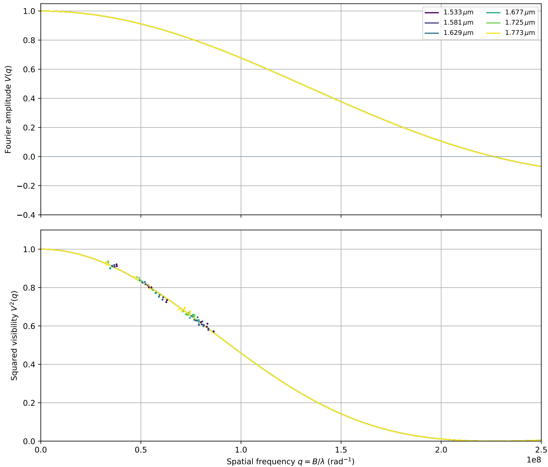
HD124850: fitted \theta_{\text{LDD}} = 1.1408 \pm 0.0051 mas
