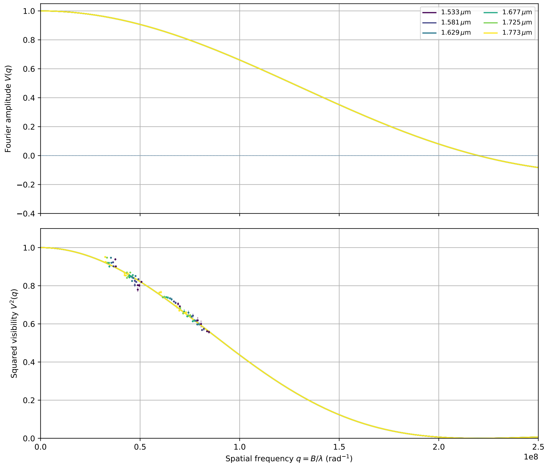
HD142860: fitted \theta_{\text{LDD}} = 1.1741 \pm 0.0138 mas
