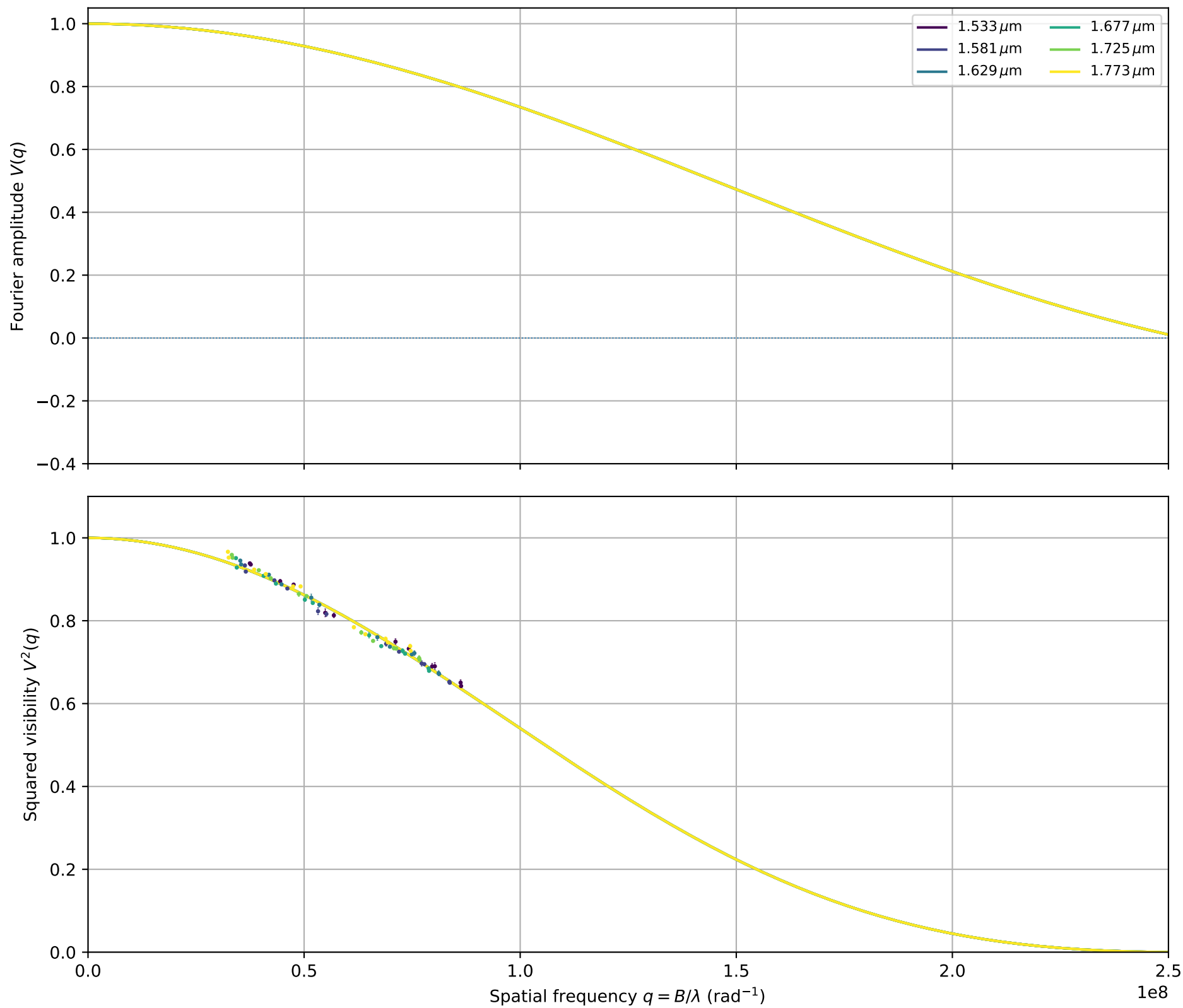
HR_2998: fitted \theta_{\text{LDD}} = 1.0301 \pm 0.0064 mas
