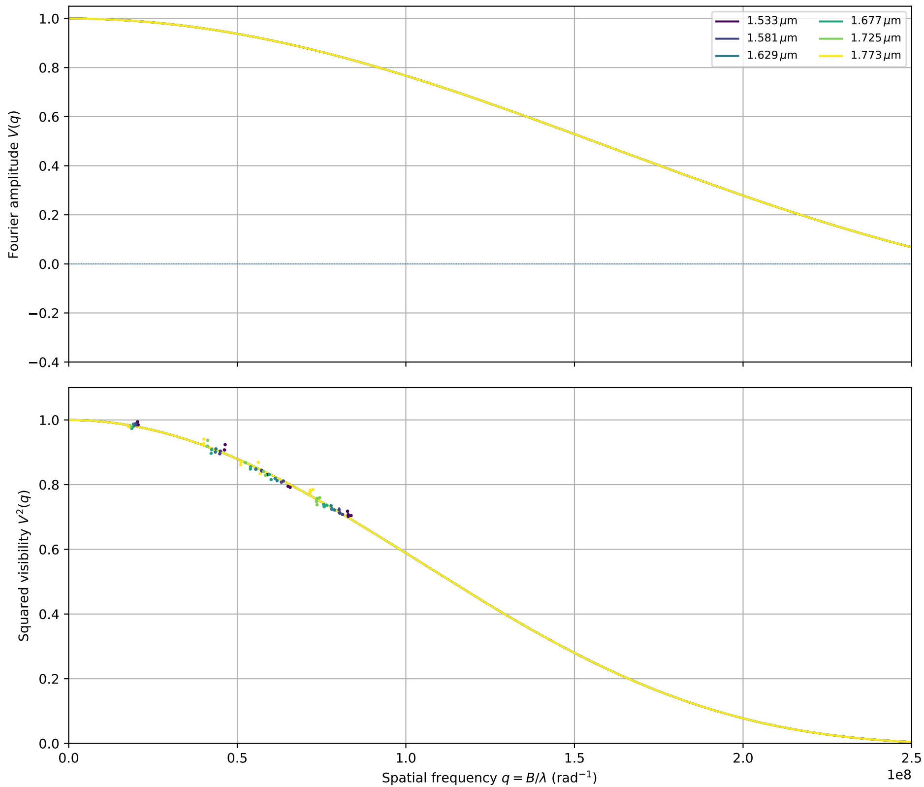
psi Vel A: fitted \theta_{\text{LDD}} = 0.9495 \pm 0.0031 mas
