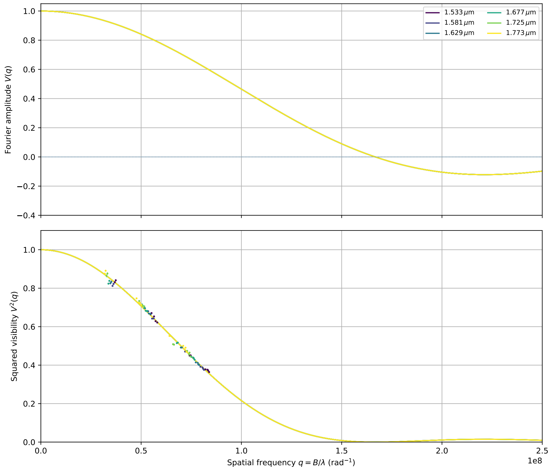
pi3_Ori: fitted \theta_{\text{LDD}} = 1.5496 \pm 0.0098 mas
