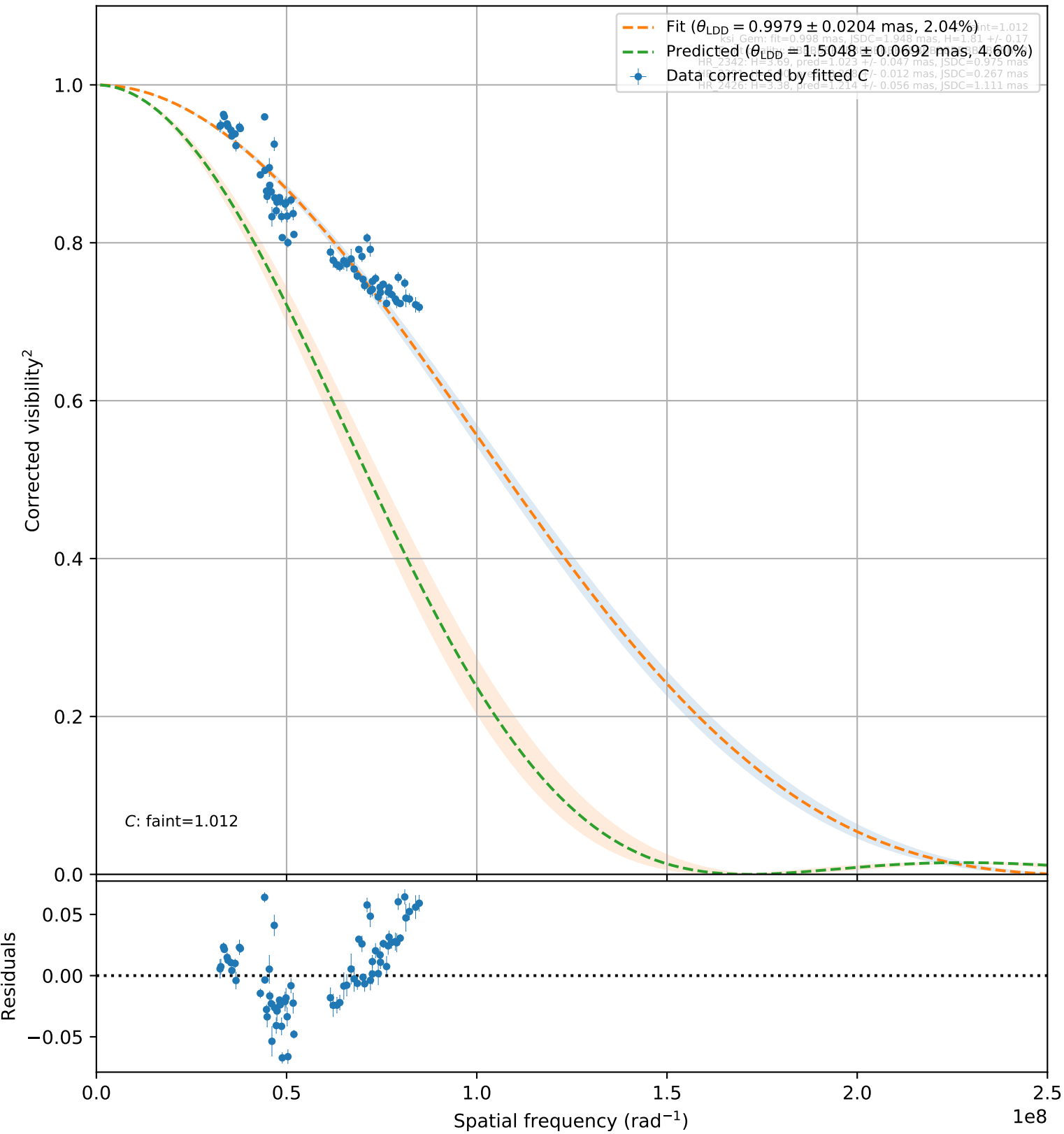
ksi_Gem (faint, 106) (72 valid vis 2 points)
