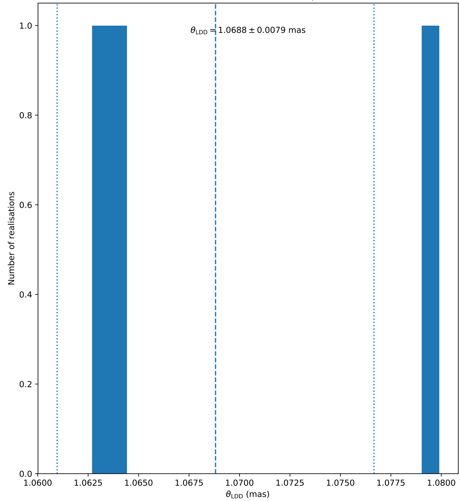
HD141004 (faint, 105) ( N_{\text{bootstrap}} = 3 )
