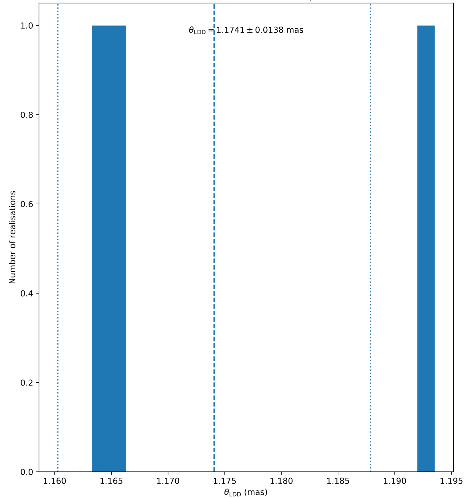
HD142860 (faint, 105) ( N_{\text{bootstrap}} = 3 )
