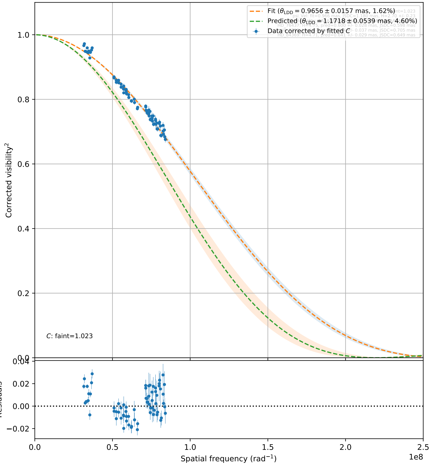
psi_Vel (faint, 106) (72 valid vis 2 points)
