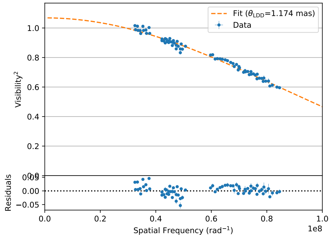
HD142860 (faint, P105)
