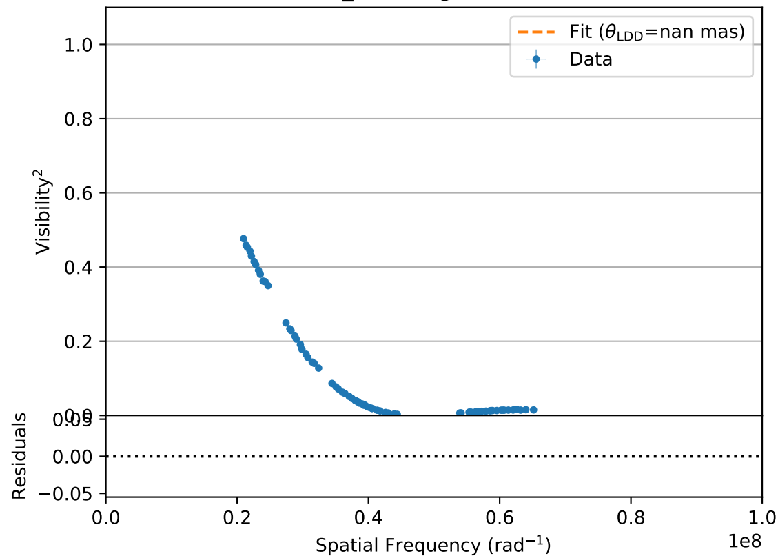
alf_CMi (bright, P106)
