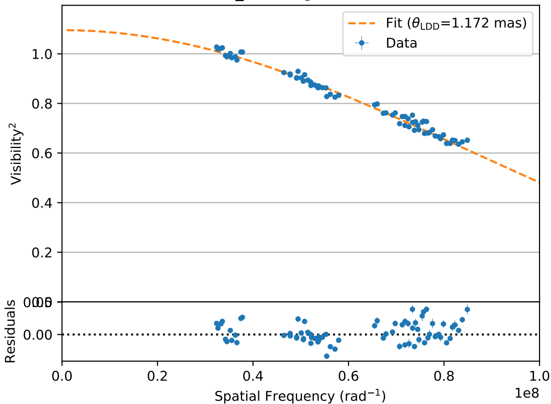
iot_Psc (bright, P104)
