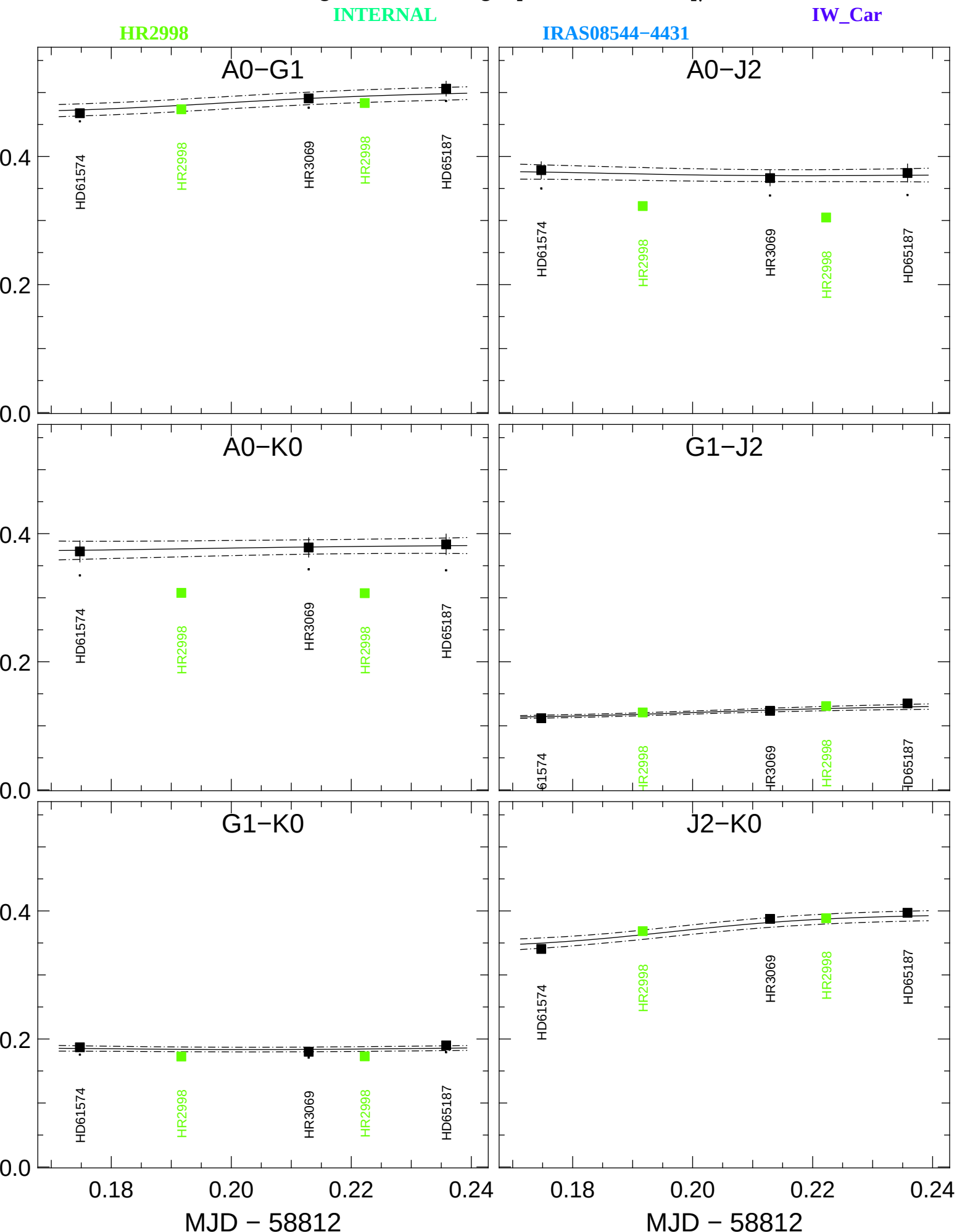
Transfer-Function vis2 (black) and Scientific vis2 (colors) averaged in the range [1.6148,1.6148] \mu\text{m}
