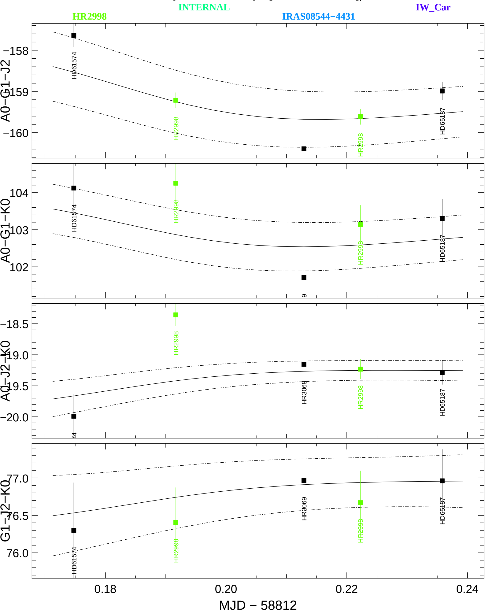
Transfer-Function t3Phi (black) and Scientific t3Phi (colors) averaged in the range [1.6148,1.6148] \mu m
