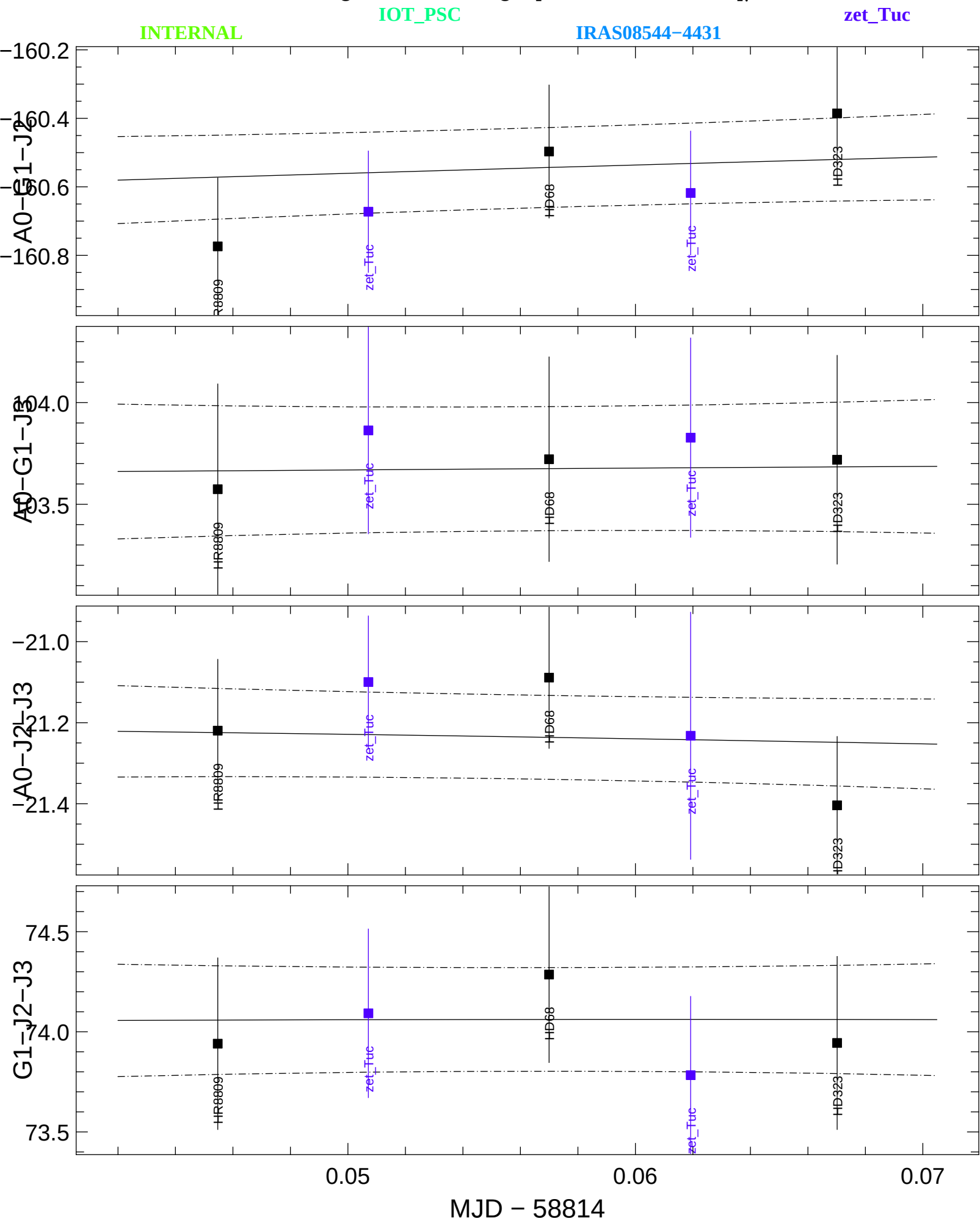
Transfer-Function t3Phi (black) and Scientific t3Phi (colors) averaged in the range [1.61591,1.61591] \mu m
