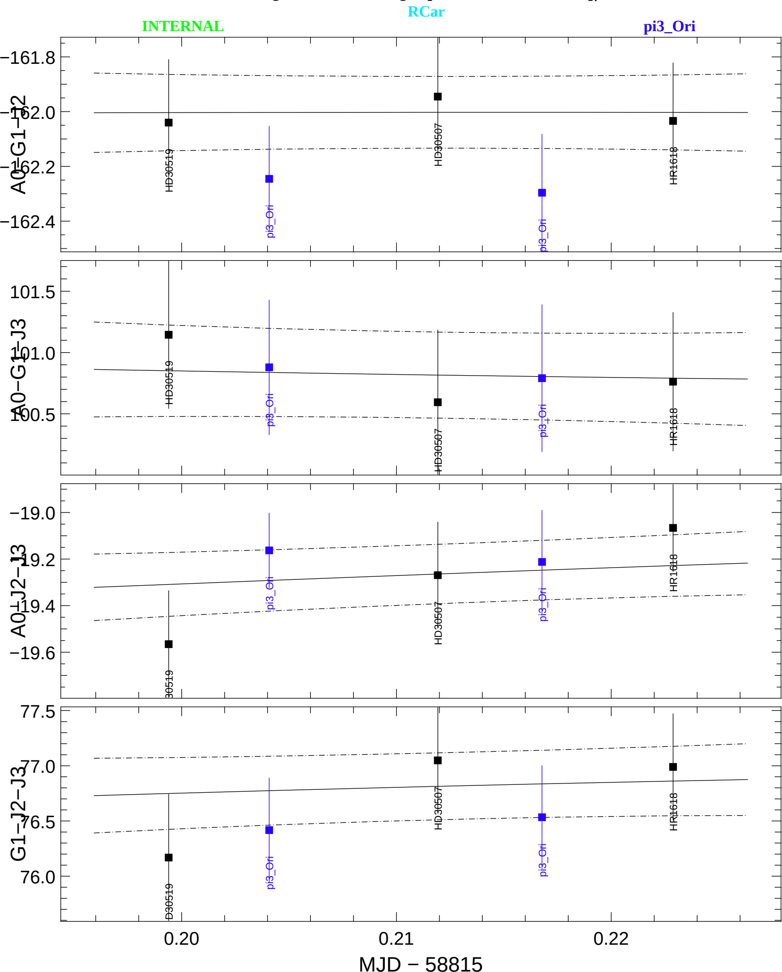
Transfer-Function t3Phi (black) and Scientific t3Phi (colors) averaged in the range [1.61531,1.61531] \mu m
