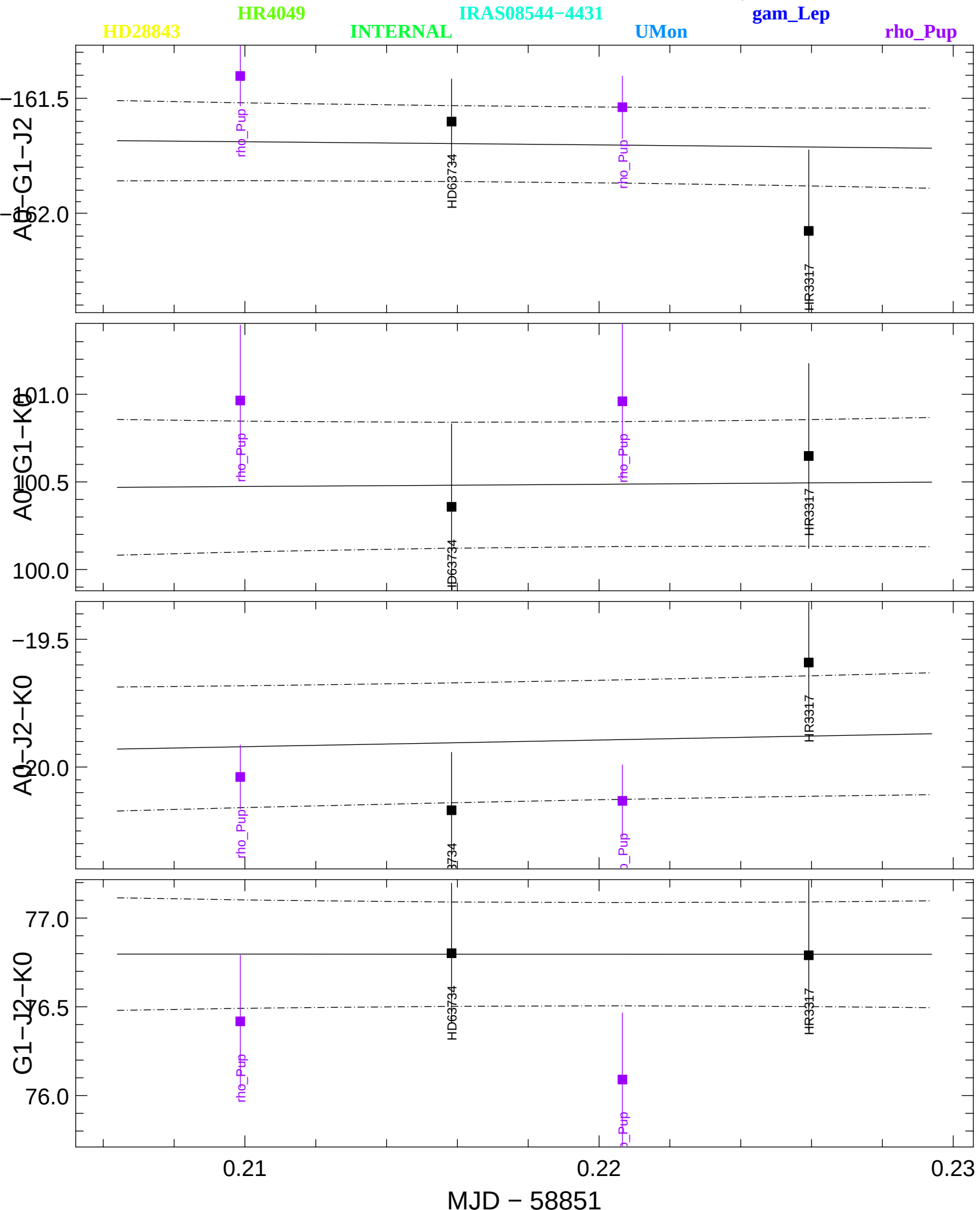
Transfer-Function t3Phi (black) and Scientific t3Phi (colors) averaged in the range [1.61555,1.61555] \mu m
