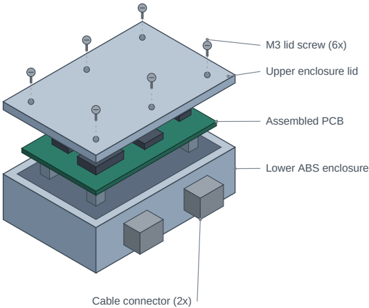
Figure 1 — CEC-120 product overview
