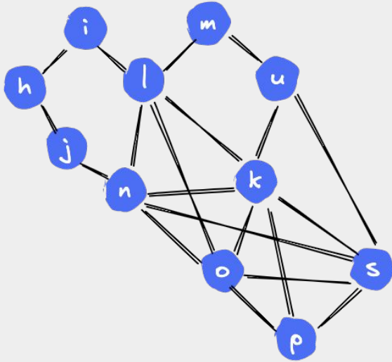
2-Core
