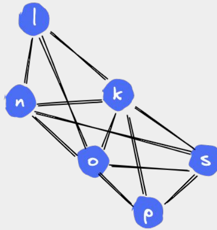
3-Core
