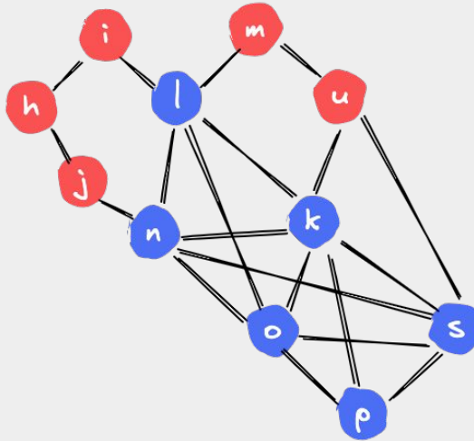
2-Shell
