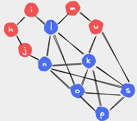
2-Shell
