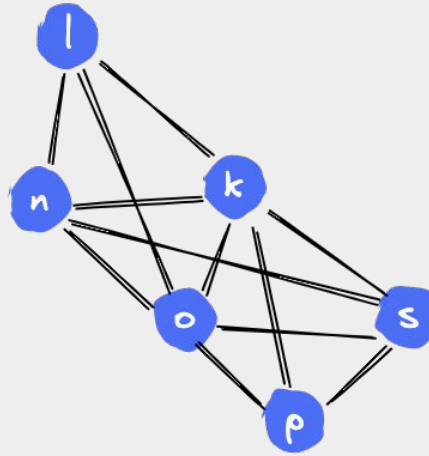
3-Core
