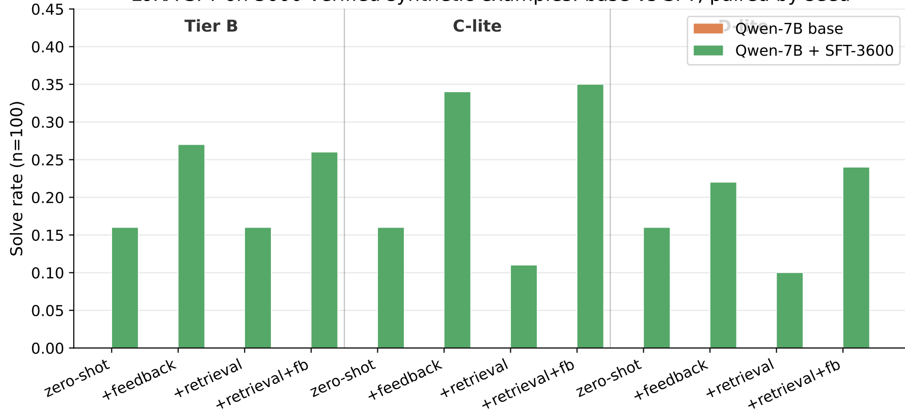
LoRA SFT on 3600 verified synthetic examples: base vs SFT, paired by seed
