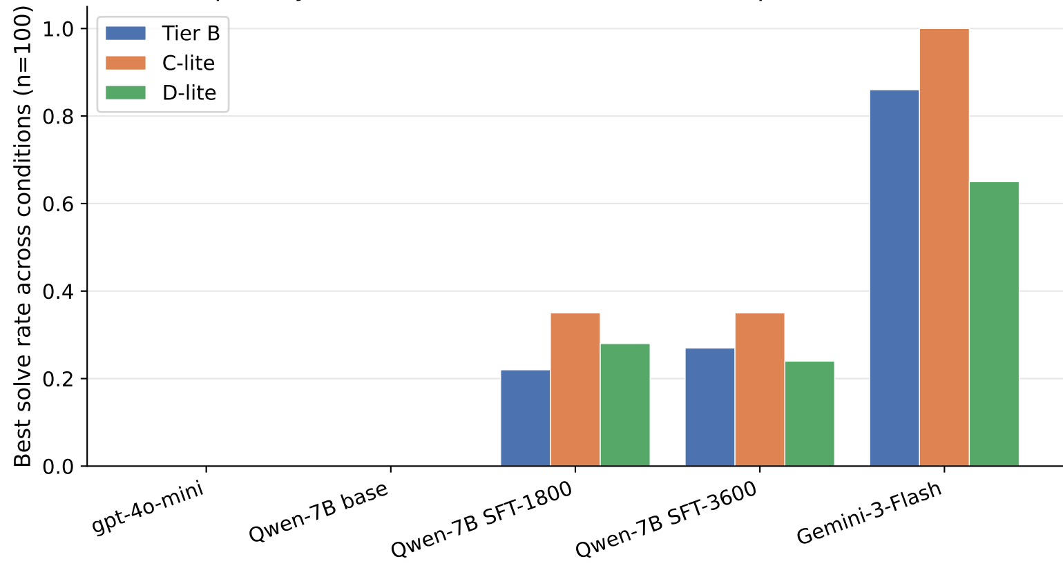
Capability ladder: best (across 4 conditions) per model × tier
