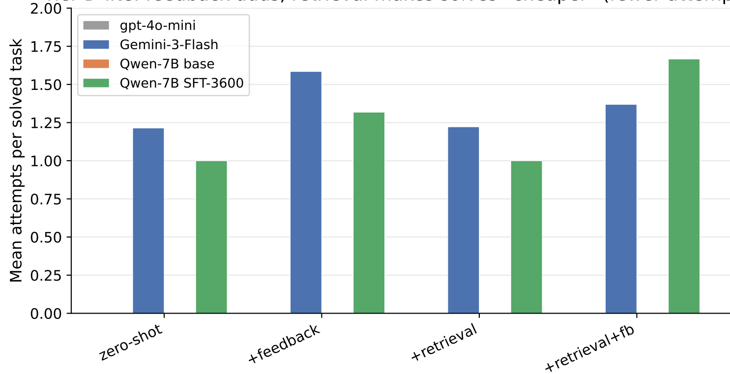
Tier D-lite: feedback adds, retrieval makes solves *cheaper* (fewer attempts)
