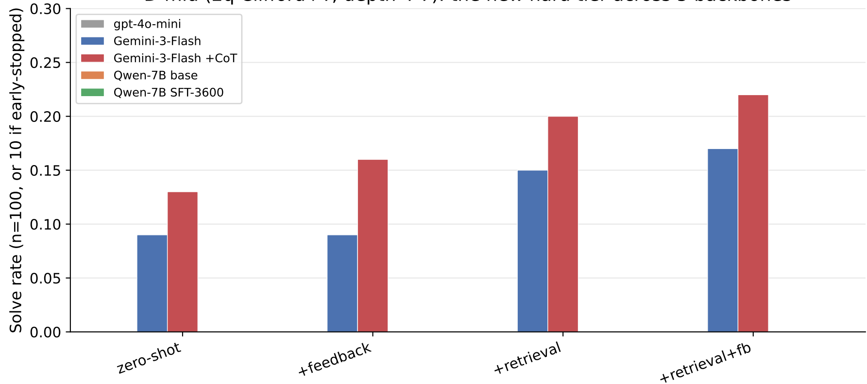
D-mid (2q Clifford+T, depth 4-7): the new hard tier across 5 backbones
