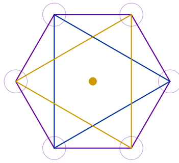
Vector Equilibrium (Cuboctaedro)
