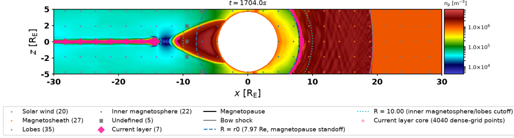
Figure 1: Extracted VDF cells, colored by ground-truth label, smoke_test run. Blue dashed circle: fitted Shue standoff r_0 . Cyan dotted circle: lobe_r_min_re . Pink dot cloud: the current-layer core’s dense-grid extent; pink diamonds: the VDF cells actually labelled current_layer .
