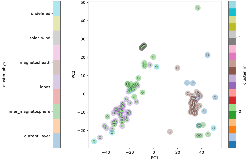
Figure 3: PCA scatter (first two principal components), smoke.test run, hermite features + moments, k = 2 .
