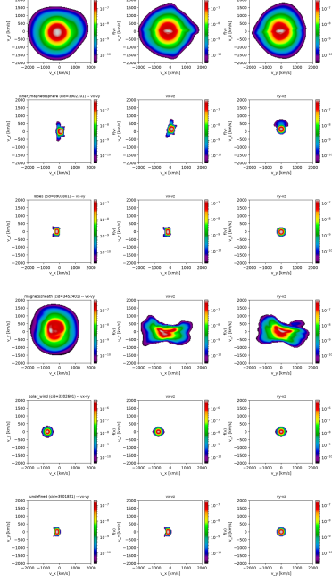
(b) Velocity-space cuts ( v_x-v_y , v_x-v_z , v_y-v_z , sliced through each VDF's own peak) of the same representatives, same order.
