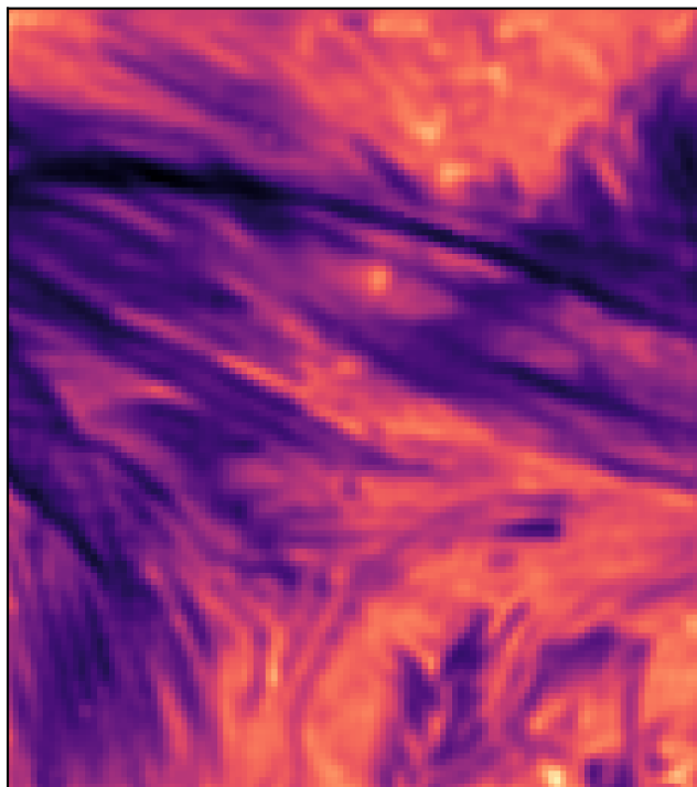
Fitted @ 6562.205 Å (idx=110)
