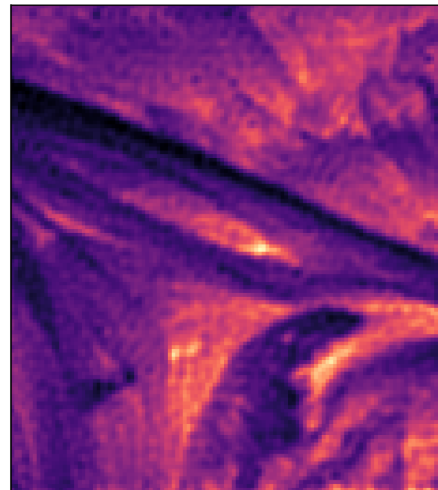
Fitted @ 6562.970 Å (idx=200)
