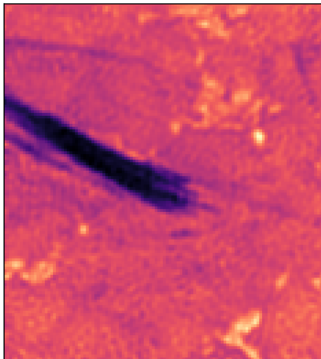
Fitted @ 6561.440 Å (idx=20)
